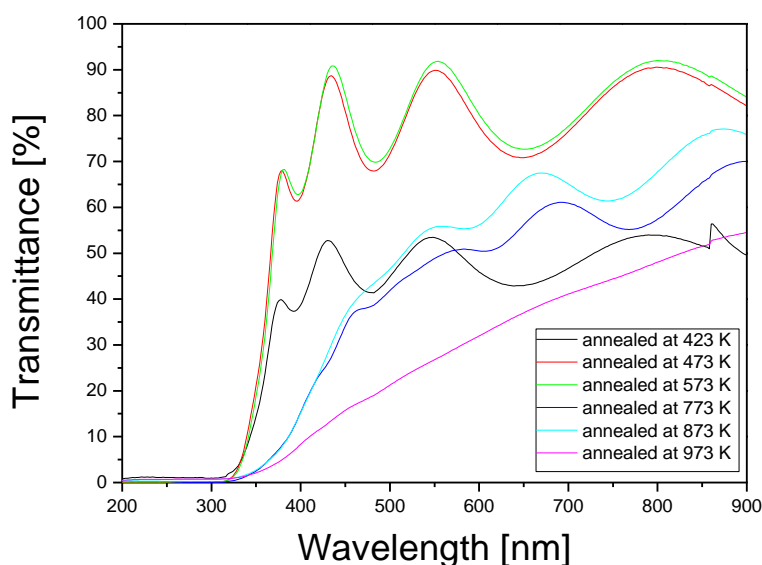
Figure 6. Transmittance measurements of the TO films annealed in the range of temperatures from 423 K to 973 K.
