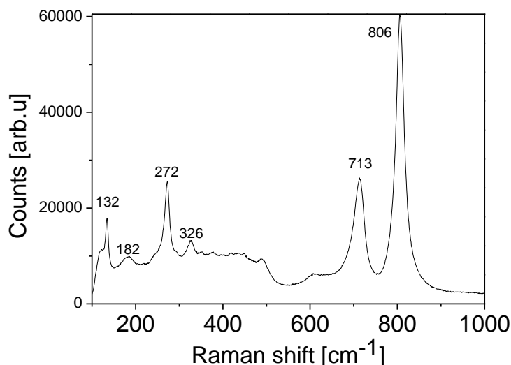
Figure 2. Raman spectra of the TO film annealed at 973 K.
