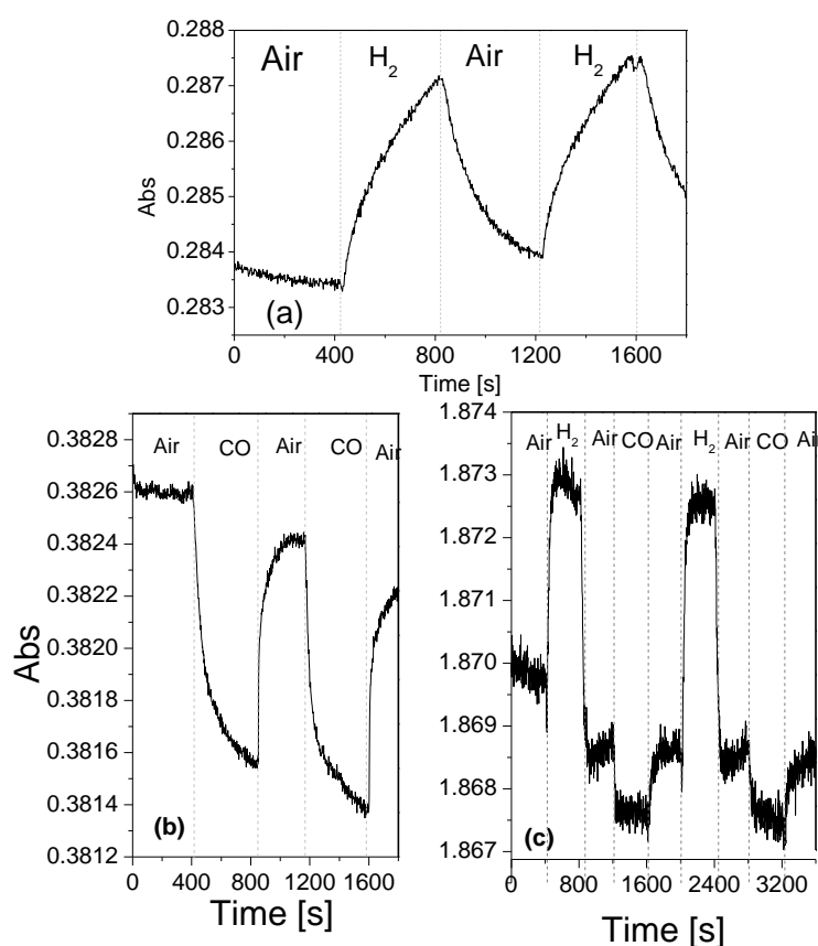
Figure 9. Time resolved absorbance change ( \Delta Abs ) tests for a Pt/ WO_3 film operated at different temperatures (a) \Delta Abs recorded at 850 nm for 1% v/v H_2 operating the film at room temperature; (b) \Delta Abs recorded at 650 nm for the 1% v/v CO operating the film at 423 K (c) \Delta Abs recorded at 340 nm for 1% v/v H_2 and 1% v/v CO operating the film at 423 K.
