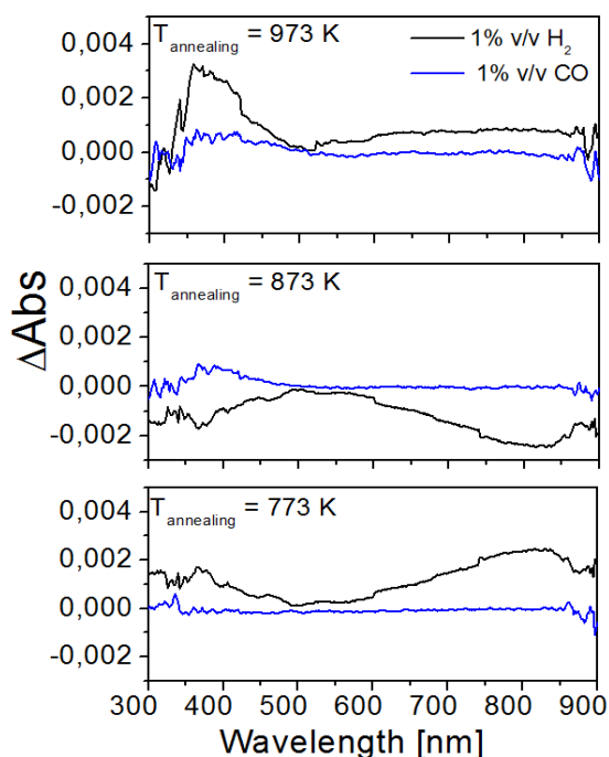
Figure 7. Optical Absorbance Change, \Delta\text{Abs} = \text{Abs}_{\text{gas}} - \text{Abs}_{\text{Air}} , curves of samples annealed at 773 K, 873 K and 973 K, for H 2 and CO at operating temperature 573 K.
