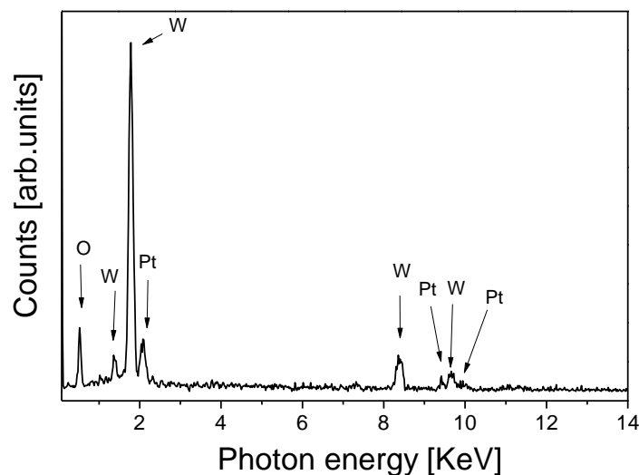
Figure 5. EDS graph of the WO 3 assisted with Pt.
