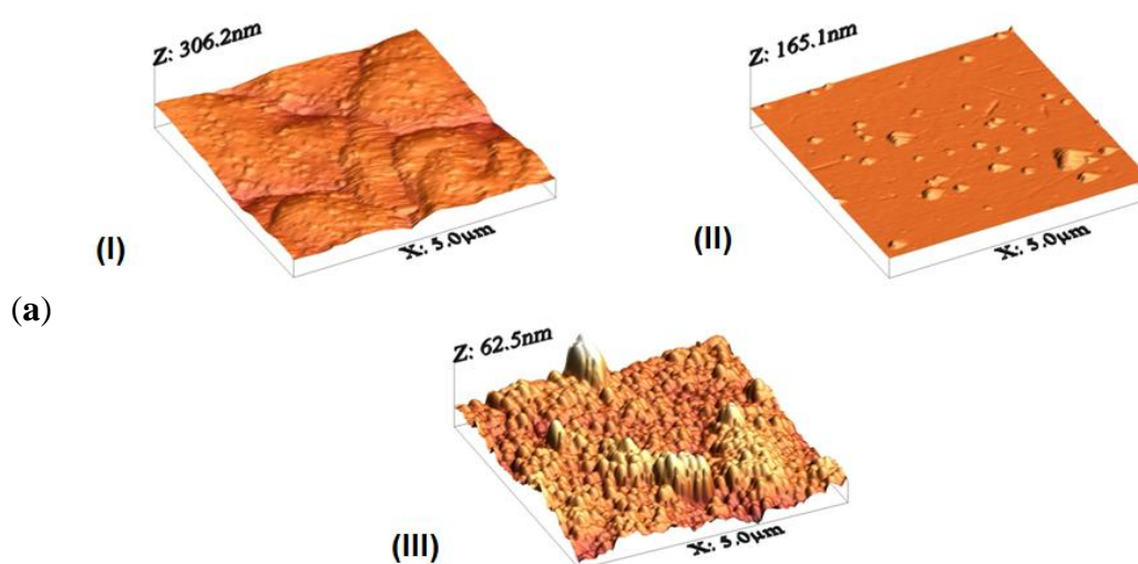
Figure 3. (a) AFM micrograph of three different samples annealed at temperatures ranging from 773 K to 973 K. I. annealed at 973 K, II. annealed at 873 K and III. annealed at 773 K; (b) AFM micrograph of four different regions of the same sample, annealed at 773 K.
