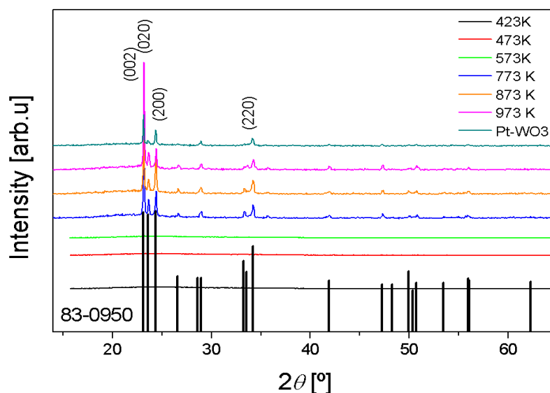
Figure 1. X-ray powder diffraction patterns of the TO films annealed in the range of temperatures from 423 K to 973 K and X-ray powder diffraction pattern of the \text{WO}_3 films annealed at 973 K with Pt nanoparticles.
