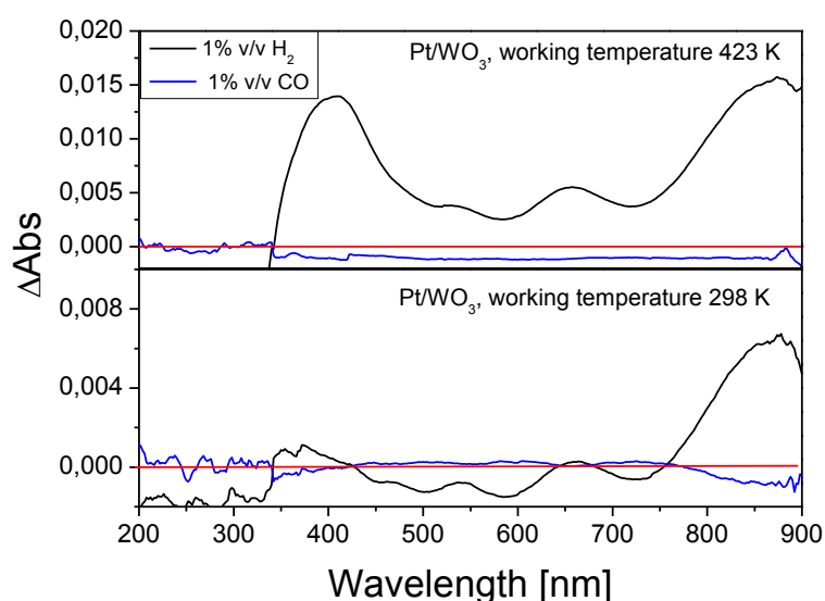
Figure 8. Optical Absorbance Change, \Delta\text{Abs} = \text{Abs}_{\text{gas}} - \text{Abs}_{\text{Air}} , curve of Pt assisted \text{WO}_3 , for \text{H}_2 and CO at 423 K and room temperature. The red line indicates the zero change in the absorption.
