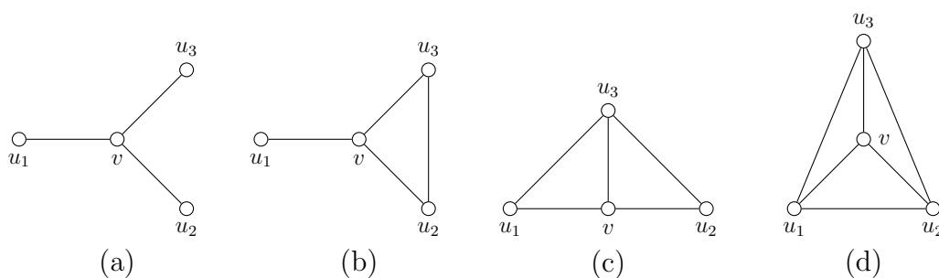
Figure 2.2: Possible cases for a vertex v with three adjacent vertices u_1, u_2, u_3 .
