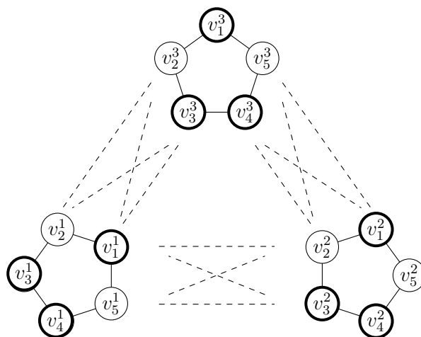
Figure 3.7: Sketch of lexicographic product K_3 \circ C_5 , where the dashed line between two cycles C_5 means that each vertex of a cycle is connected to all vertices of the other cycle. The vertices represented by thick lines form a 2-adjacency basis of each copy of C_5 .
