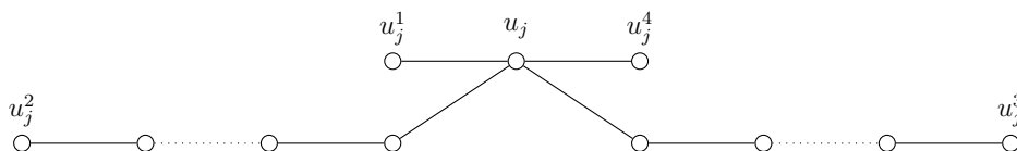
Figure 4.2: The subgraph associated to the clause Q_j .
