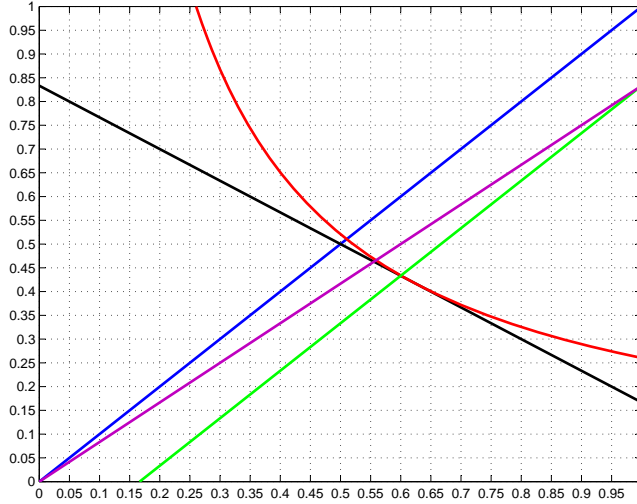
Figure 3: Main bargaining solutions: N (red), KS (purple), E (blue) and EL (green).
