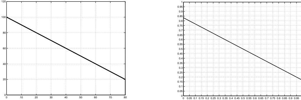
Figure 1: A claims problem ( E = 100 , c = (80, 120) ) and its associated bargaining-in-proportions problem . The main difference is the gradient of the Pareto boundary, which is -1 in the claims problem, and -8/12 in the associated bargaining-in-proportions problem.
