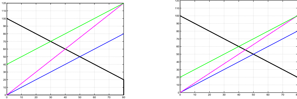
Figure 2: Claims rules ( CEA (blue), CEL (green), P (pink), on the left hand side) and truncated claims rules ( CEA (blue), CEL^T (green) and P^T (pink), on the right hand side). Note that CEA is invariant to claims truncation.
