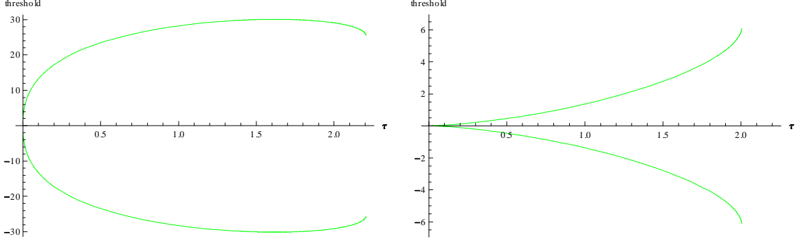
Figure 1: The optimal two-sided threshold strategy for varying time: If a deviation increases the noise (left) the set S is the union of the signals above and below the top and bottom curves, respectively. If a deviation decreases the noise (right) the set S is the intersection of the signals below and above the top and bottom curves, respectively.
