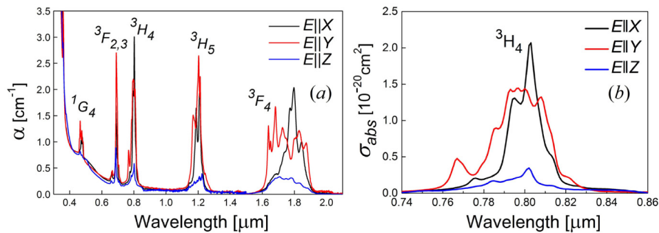
Fig. 2. (a) RT polarized absorption of 0.89 at.% Tm:MgWO _4 , \alpha is the absorption coefficient; (b) RT absorption cross-section, \sigma_{\text{abs}} , spectra corresponding to the ^3\text{H}_6 \rightarrow ^3\text{H}_4 transition.
