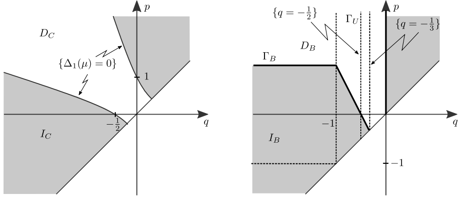
Figure 2: Bifurcation diagram of the period function at the inner boundary (left) and at the outer boundary (right), according to Theorem B and Theorem 1.3, respectively.
