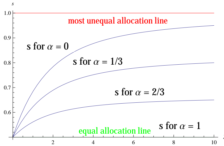
Figure 1: The universal share of the total resource s as a function of \lambda for different values of \alpha . Note that s converges to the equal allocation line for \alpha \uparrow 1 , but does not converge to the most unequal allocation line for \alpha \downarrow 0 unless \lambda \uparrow \infty .
