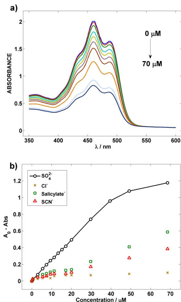
Fig. 3 (a) Spectra of the sulphate sensor in 10 mM HAc/MgAc at pH 4 upon additions of \text{Na}_2\text{SO}_4 . (b) Calibration curves with the difference in absorbance at 459 nm ( \Delta\text{Abs} ) for \text{SO}_4^{2-} and other anions.
