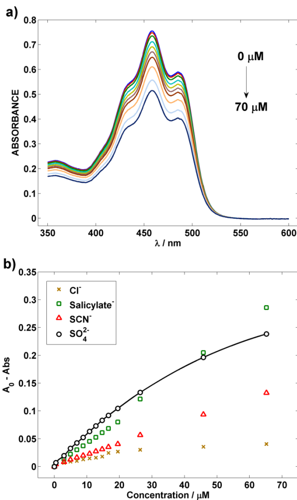
Fig. 2. (a) Spectra of the blank sensor in 10 mM HAc/MgAc at pH 4 upon additions of \text{Na}_2\text{SO}_4 . (b) Calibration curves with the difference in absorbance at 459 nm ( A_0 - \text{Abs} ) for \text{SO}_4^{2-} and other anions.
