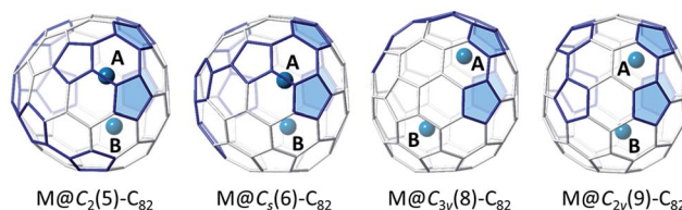
Fig. 6 Structures for the EMFs M@C_{82} ( M = Ba, La, Hf, U ) showing positions A and B of the metal atom for M@C_{2(5)}-C_{82} , M@C_{s(6)}-C_{82} , M@C_{3v(8)}-C_{82} and M@C_{2v(9)}-C_{82} . Bonds forming pyracylene units are highlighted in blue. Pentagons of pyracylene units fixed at the same position are filled in blue.
