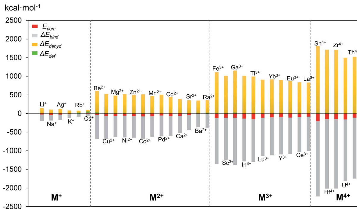
Fig. 7 Complexation energy E_{\text{com}} (in \text{kcal mol}^{-1} ) of M^{n+} encapsulated in \text{Pd}_{12}\text{L}_8 ( \text{L} = \text{PhAs} ) host shell and its decomposition terms \Delta E_{\text{dehyd}} , \Delta E_{\text{bind}} and \Delta E_{\text{def}} .
