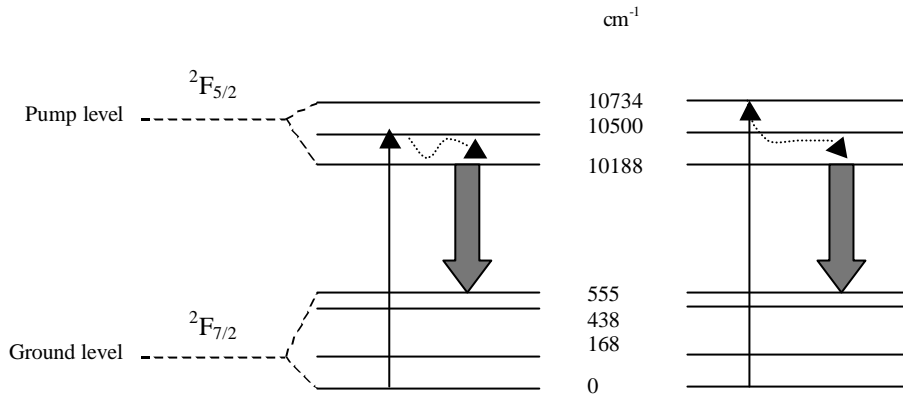
Figure 5.2 Pump-laser schemes of Yb^{3+} in KYbW at two pump wavelengths, at 963 nm (left) and at 922 nm (right)
