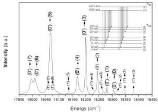
Figure 4.13 Low temperature green emission of \text{Er}^{3+} in \text{KYbW}
