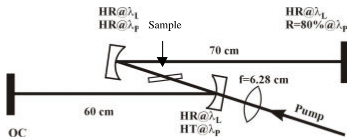
Figure 2.7 Laser set-up for the CW experiments on \text{Yb}^{3+} -doped KLuW samples
