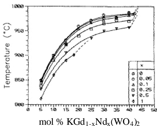
Figure 4.1 Solubility curves of the system KGd_{1-x}Nd_x(WO_4)_2 - K_2W_2O_7 from reference 124
