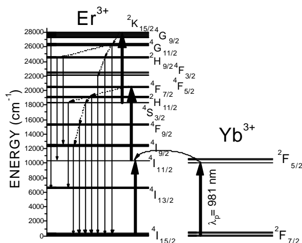
Figure 4.15 Scheme of the pump-emission and energy transfer for the generation of the ultraviolet and visible emissions of \text{Er}^{3+} in \text{KRE} co-doped with \text{Yb}^{3+}
