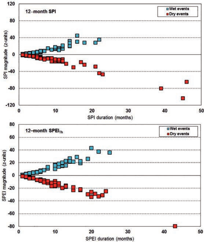
Figure 5. Behaviour of identified droughts and wet events in Barcelona (1787-2014) according to the magnitude reached for each event related with the duration in months by using 12-month SPI and SPEI 7h series.
