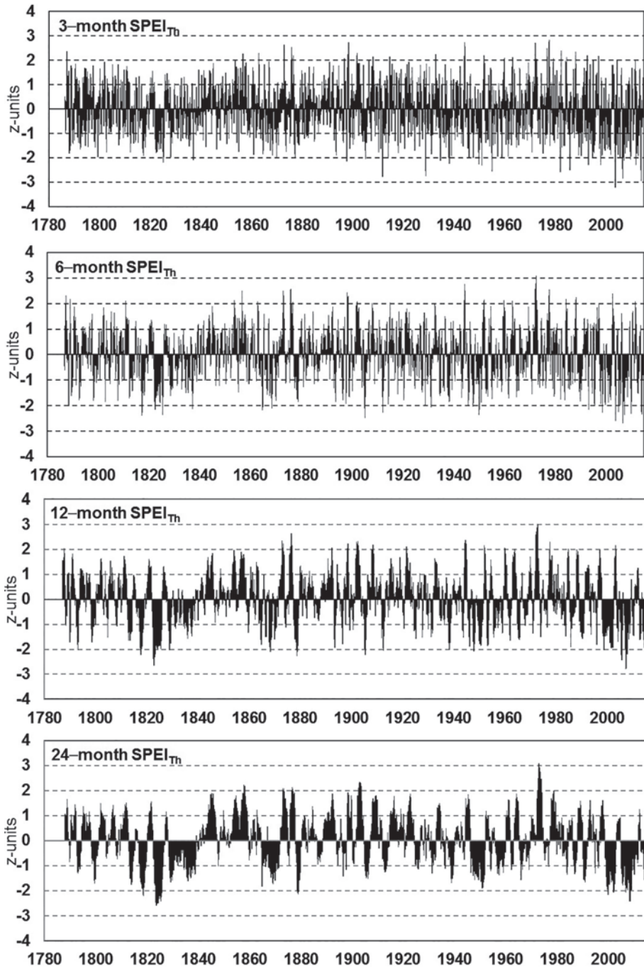
Figure 3. Drought variability from the 3-, 6-, 12- and 24-month SPEI Th computed for Barcelona (1787-2014).
