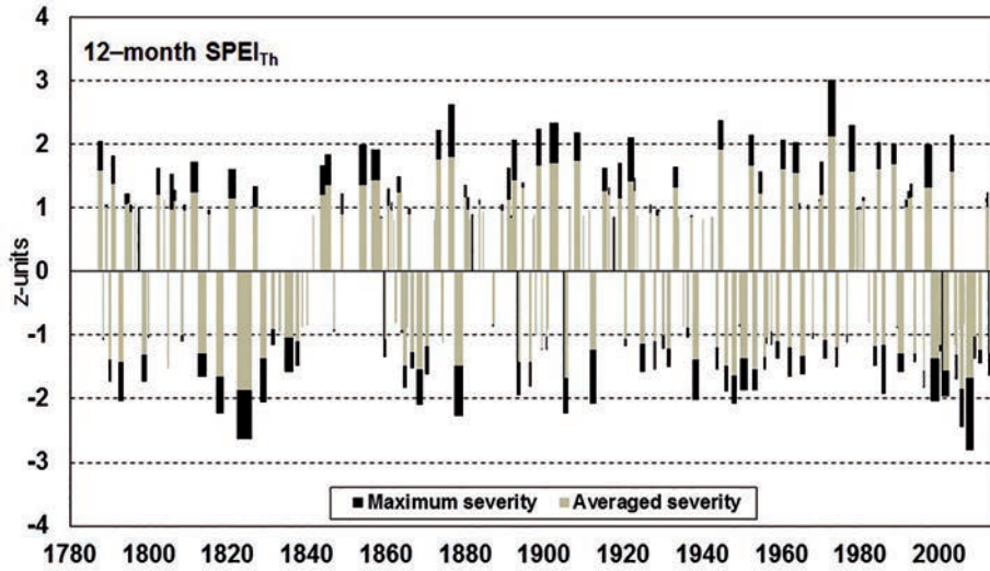
Figure 4. Droughts and wet events identified for Barcelona (1787-2014) by using the 12-month SPI and SPEI Th series. Black bars (or grey bars) are referred to the maximum severity (or average severity) reached for each drought and wet event and bars width's are proportional to duration in months.
