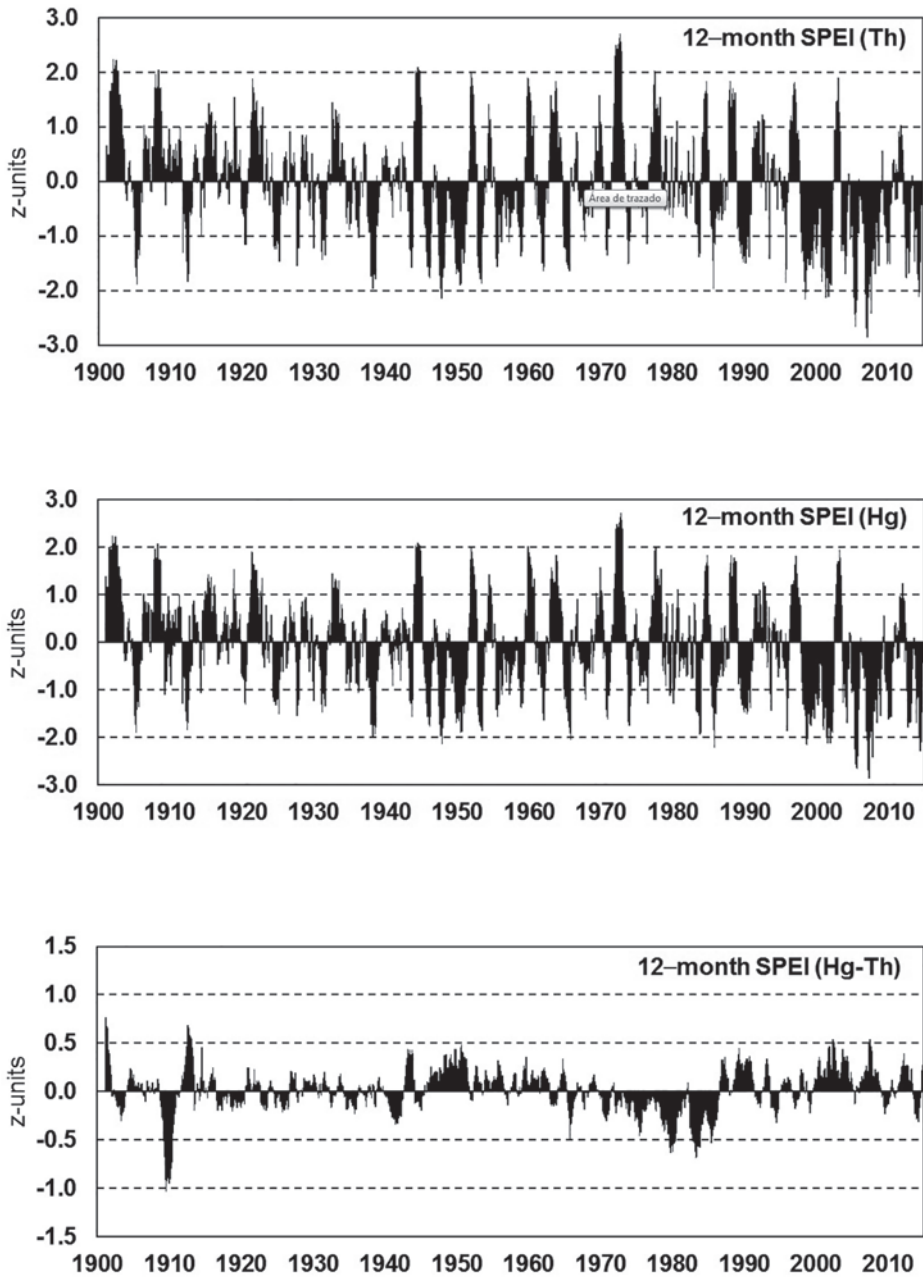
Figure 1. 12-month SPEI time series for Barcelona (1901-2014) based on the Thornthwaite (Th) and Hargreaves (Hg) reference evapotranspiration equations and differences between both ETO estimation methods (Hg-Th).
