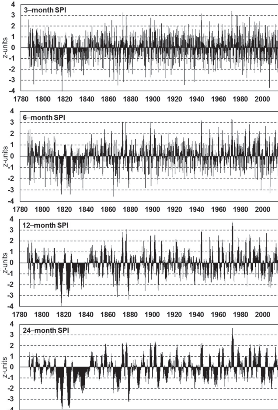
Figure 2. Drought variability from the 3-, 6-, 12- and 24-month SPI computed for Barcelona (1787-2014).
