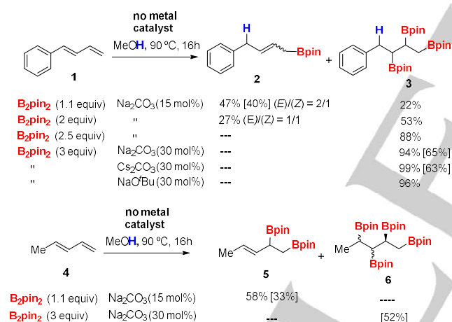
Scheme 2. Transition-metal-free borylation of trans -1-phenyl-1,3-butadiene and trans -1-methyl-1,3-butadiene.
