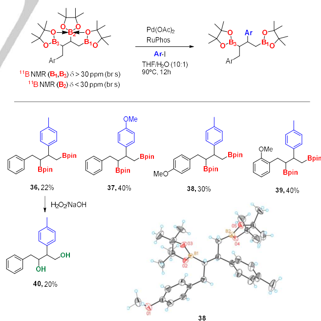
Scheme 4. Cross-coupling of 1,2,3-triborated products with 1-iodo-4-methylbenzene and 1-iodo-4-methoxybenzene in the presence of \text{Pd}(\text{OAc})_2/\text{RuPhos} , and in situ oxidation of 36 . X-Ray Diffraction Data for compound 38 .
