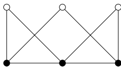
Figure 1. A graph H belonging to \mathcal{G} . The set of black-coloured vertices forms a \gamma_{st}(H) -set
