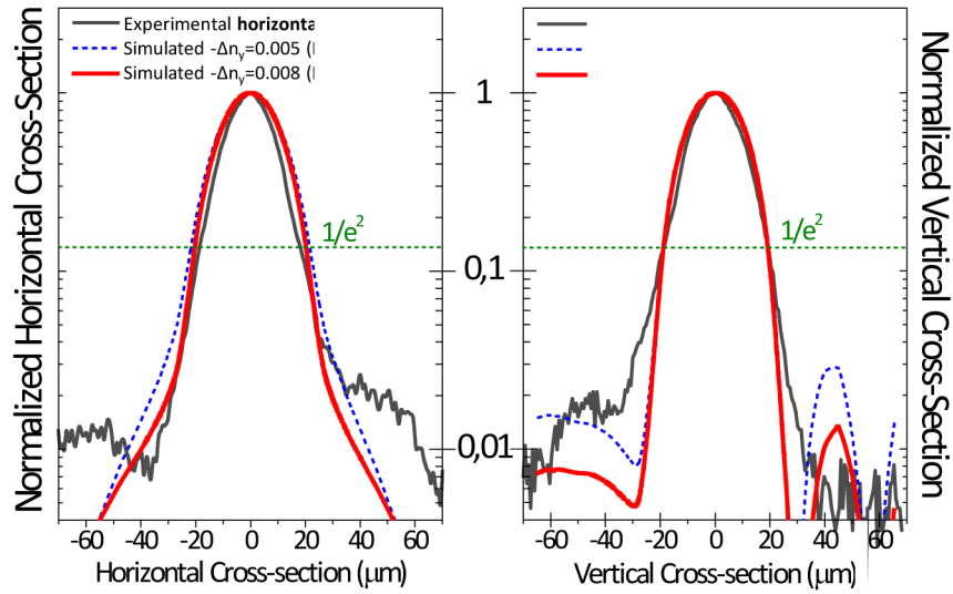
Fig. 4. Comparison of near field TE mode cross sections of simulations and experiment. Horizontal cross sections are shown on the left and vertical cross sections are shown on the right. The best matching between simulated and measured cross sections was obtained for an index change inside tracks of \Delta n = -0.008 .
