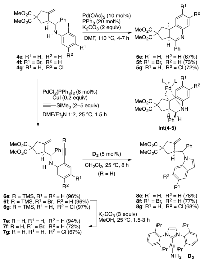
Scheme 2. Transformation of Adducts 4e–g into Tetrahydro-1 H -cyclopenta[ c ]quinoline and Indole Derivatives via Pd(0)-Catalyzed Cross-Coupling and Au(I)-Catalyzed Cyclization
