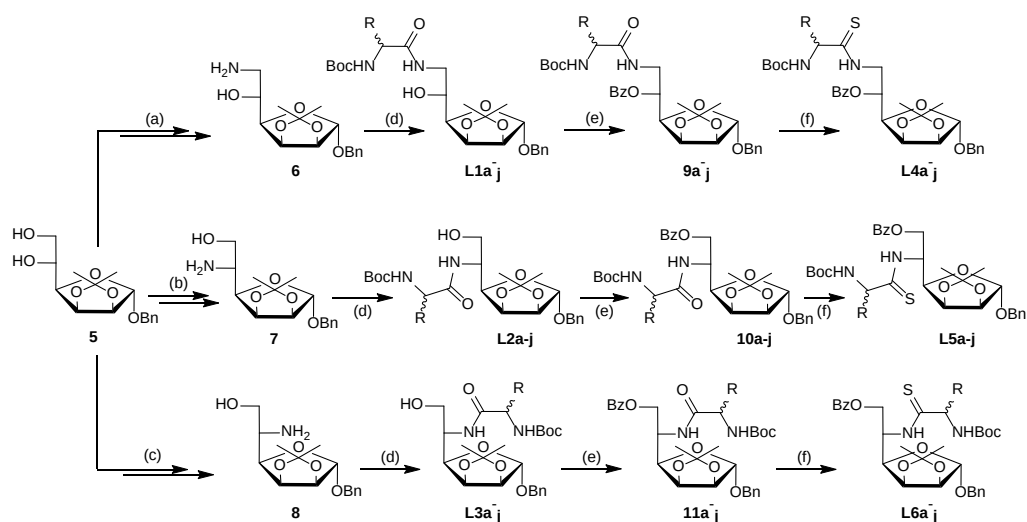
Scheme 1. Synthesis of hydroxyamide and thioamide ligands L1-L6a-j . (a-c) See Supporting Information for details. (d) N-Boc-protected \alpha -amino acid/ t BuOCOC/NMM/THF/-15 °C. (e) BzCl/ \text{NEt}_3 /DMAP/ \text{CH}_2\text{Cl}_2 /0 °C to rt. (f) Lawesson's reagent/THF/60 °C.
