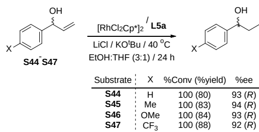
Scheme 2. Tandem isomerization/ATH reactions of allylic alcohols using Rh- L5a
