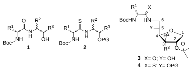
Figure 1. General structure of hydroxyamide ligands 1 , thioamide ligands 2 and sugar-based hydroxyamide 3 and thioamide ligands 4
