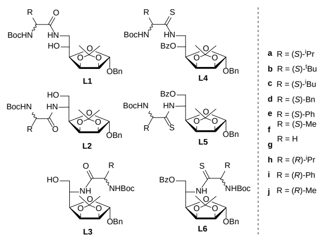
Figure 2. Hydroxyamide and thioamide ligands L1-L6a-j
