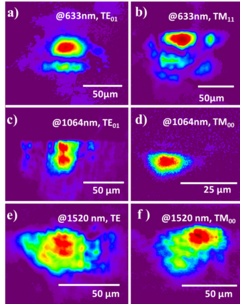
Fig. 9. (a) Near field image of the TE 01 mode at 633 nm of a straight WG, (b) Near field image of TM 11 mode at 633 nm of a straight WG, (c) Near field image of the TE 01 at 1064 nm of a straight WG, (d) measured near field image of the TM 00 at 1064 nm of a straight WG, (e) Near field image of the TE mode at 1520 nm of a straight WG, (f) Near field image of the TM 00 mode at 1520 nm of a straight WG.
