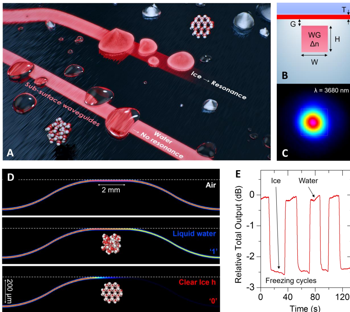
Figure 1. Mid-IR water ice phase surface sensor. (A) 3D rendered, conceptual view of the photonic sensor working mechanism. Credit: A. Trujillo. When water droplets are present on the sensor surface detection occurs by means of resonant light transfer to droplets whose index of refraction produces a phase matching condition implying a sudden dip on transmitted light. By spectrally tuning light across the OH vibrational band of water the phase state of the water layer is obtained. Since waveguides propagate below surface the sensor is immune to erosion or scratches smaller than its depth gap (B) Sensor design cross-section parameters (typical values W=15 \text{ }\mu\text{m} , H=15 \text{ }\mu\text{m} and G=5 \text{ }\mu\text{m} ) which can be changed to maximize the light coupling sensitivity to a given layer thickness T (from \sim 100 \text{ nm} to \sim 500 \text{ }\mu\text{m} ). (C) Measured near-field of the waveguide output at 3.68 \text{ }\mu\text{m} wavelength. (D) Electromagnetic beam propagation simulations of light travelling the 2 \text{ mm} long sensing waveguide for air, room temperature water and clear -7 \text{ }^\circ\text{C} homogenous ice surface layers. (E) First tests on experimental detection of freezing cycles of a water droplet with the glass sensor temperature controlled by a peltier unit and detection with a thermal power meter. The measured output intensity is evaluated as relative output power (dB) between ice and liquid water states.
