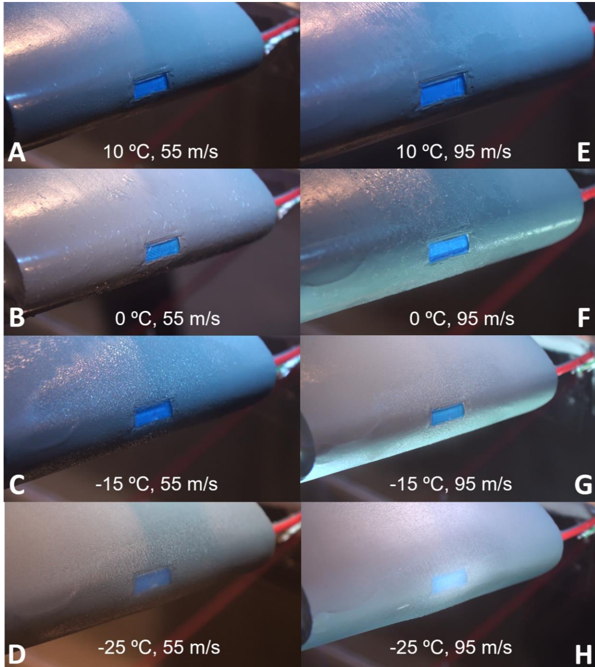
Figure 6. Wing model leading edge appearance for various temperatures and wind speeds inside the IWT. Only in the case of -25 °C and 95 m/s air speed can the first layers of ice be detected by the naked eye.
