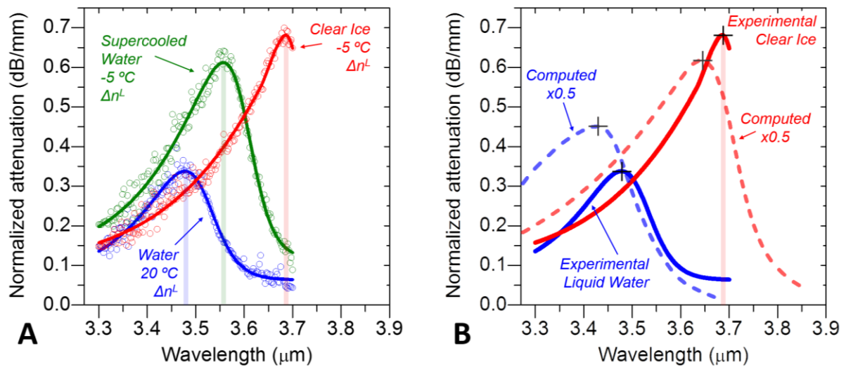
Figure 3. Experimental spectral fingerprints for warm water, SCW and clear ice with a low contrast ( \Delta n^L ) waveguide sensor. (A) Experimental normalized attenuation spectra for deionized water drop at 20 °C (blue data), and at -5 °C for both its SCW (green data) and solid state (red data). Solid lines are best fits to experimental points. Data noise is mostly arising from random output power oscillations of the tunable mid-IR OPO laser used for the experiments. Peak attenuation wavelengths are marked for each water phase state. (B) Evaluation of the matching between experimental normalized attenuation sensor data (asymmetric peak fits) and BPM simulations. Experimental data is the same as in (A), simulations used same water index of refraction data as in Figure 2, and normalized attenuation is divided by two. Good qualitative agreement on the powerful selectivity on ice against water is found, which validates the sensor 3DLW fabrication technique.
