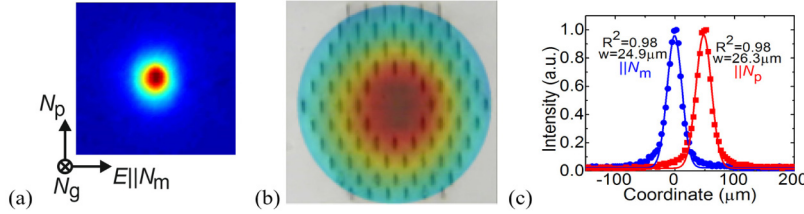
Fig. 9. Spatial profile of the output laser mode from the fs-DLW hexagonal cladding Tm:KLuW channel waveguide laser ( T_{OC} = 30\% , P_{abs} = 188 mW ): (a) 2D profile measured in the far-field, E is the laser polarization; (b) spatial overlap of the waveguide cross-section and the reconstructed beam profile at the output facet of the waveguide; (c) the corresponding 1D profiles of the laser mode in the horizontal ( \parallel N_m ) and vertical ( \parallel N_p ) directions.
