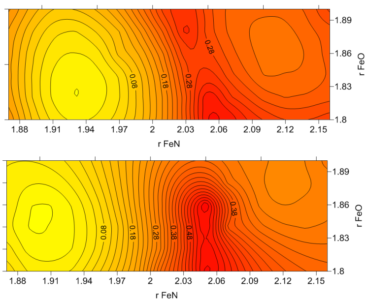
Figure 4: CASPT2 potential energy surface as function of the Fe-N and Fe-O distances (Å) of the lowest electronic state in the complexes [Fe(qsal) 2 ] + (top) and [Fe(pap) 2 ] + (bottom). Energies (in eV) are relative to the total energy of the LS minimum.
