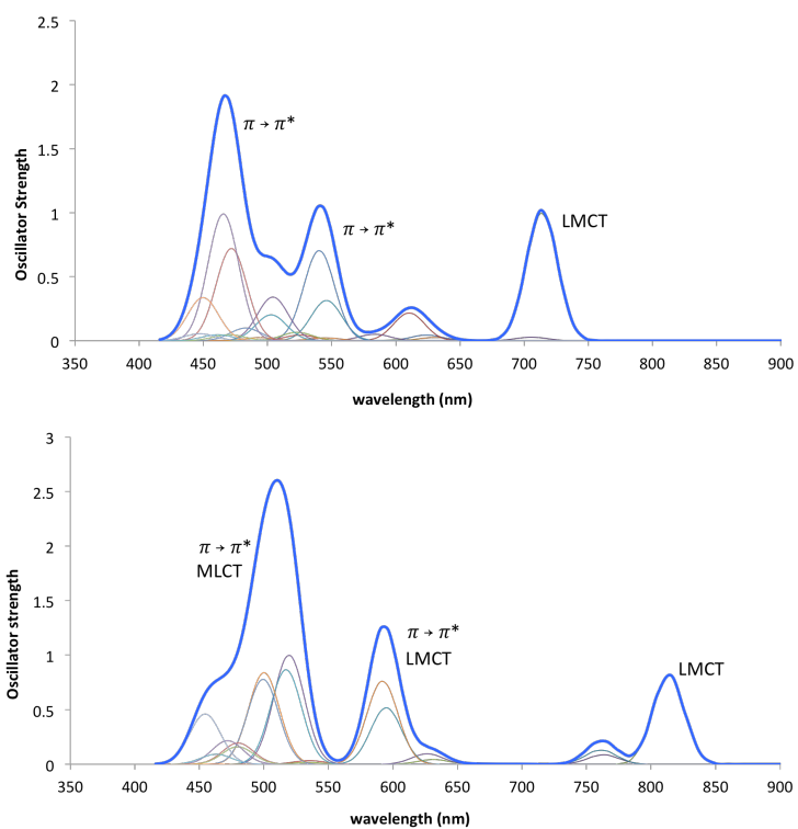
Figure 6: B3LYP* absorption spectrum of [Fe(qsal) 2 ] + (top) and [Fe(pap) 2 ] + (bottom). The individual transitions (thin lines) are represented by a Gaussian function ( bw = 40 nm). Oscillator strength in arbitrary units.
