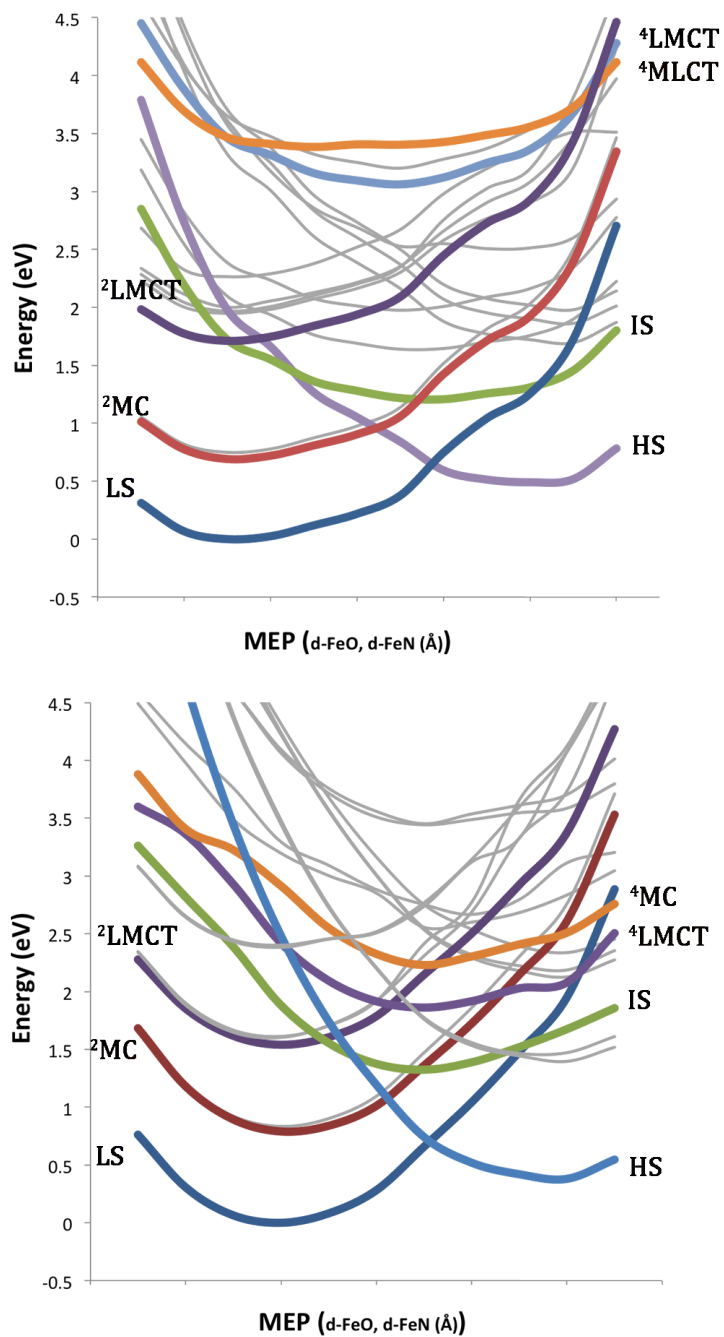
Figure 8: B3LYP* potential energy curves for a collection of electronic states along the quasi-MEP of the complexes [Fe(qsal) 2 ] + and [Fe(pap) 2 ] + .
