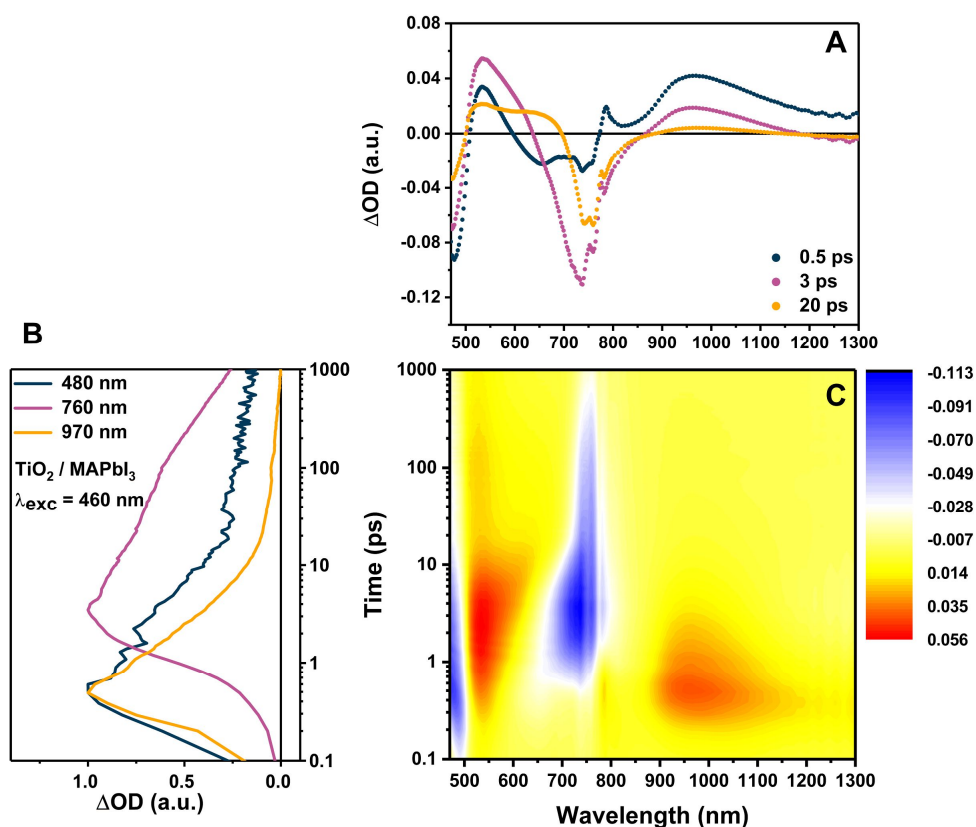
Figure 4.15. FsTA spectra of TiO 2 /MAPbI 3 films with \lambda_{\text{exc}} = 460 nm. Differential absorption spectra (A) with time delays of 0.5 ps (blue), 3 ps (purple), and 20 ps (orange). Time absorption profiles (B) at 480 nm (blue), 760 nm (purple), and 970 nm (orange) showing the electron injection into the TiO 2 layer.
