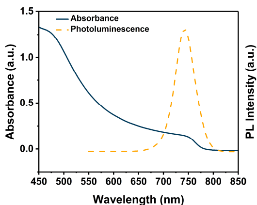
Figure 3.7. UV-Vis absorption spectra of the \text{MAPbI}_3 perovskite. It is clearly observed the two different absorbance features at 760 and 480 nm.
