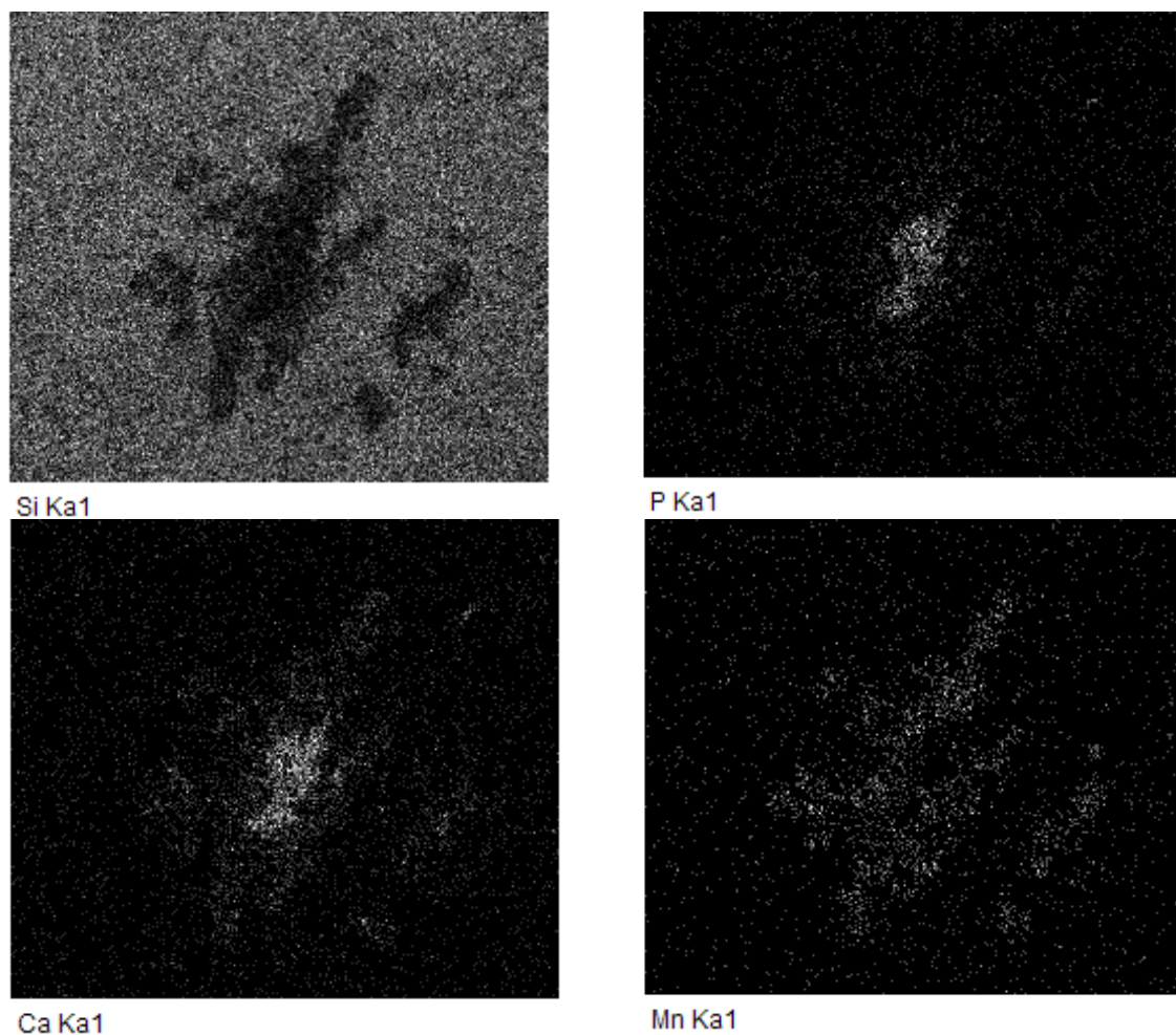
Figure 14: Showing the different elements extracted with the EDX of the residue in figure 11. Si (the flint), P and Ca (bone residue) and Mn (black residue surrounding the bone residue)
