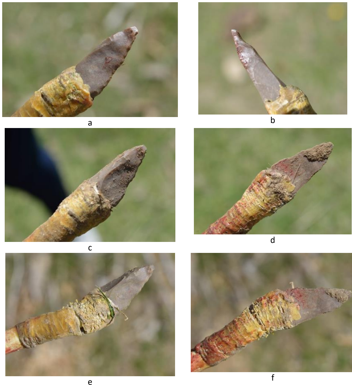
Figure 4.2: Zaragoza no. 1 (arrowhead, 8 shots were performed) (a-b) tip fracture and blood residue on the tool surface, (c-d) in attempt 3 tool penetrate inside the ground till the hafting area; (e-f) attempt 8 the tool misplaced on the haft after hitting the ground
