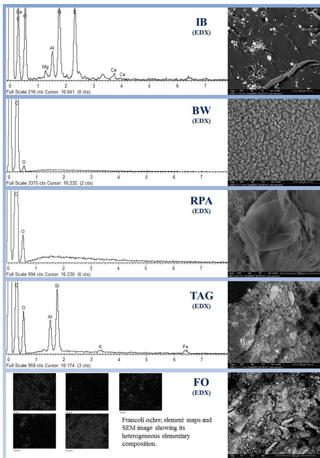
Figure 2: Element graph map generated under ESEM with EDX; 1) IB (Khorramabad Bitumen, Iran), 2) BW (Beeswax), 3) RPA (Pistachio resin, Iran), 4)TAG (Adire tree pitch) and 5) FO (Francoli Ocher, Spain)
