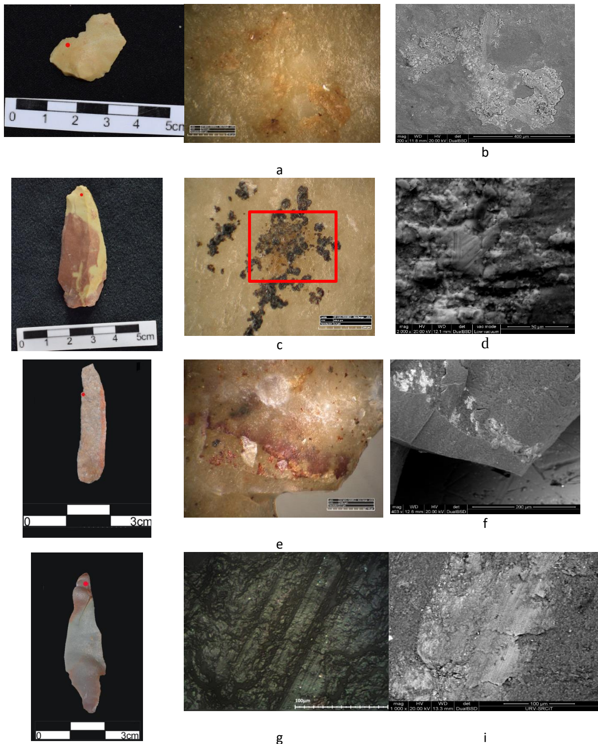
Figure 11: left column top to bottom showing the tools with the location of the residue and on the right two rows theirs magnified details. (a,b) KLD-E6-5II-912 (flake) (a) amorphous pale brown colour residue with striation under 3D DM at 400x (Mid-Range lens); (b) same location under SEM with EDX at 521x; (c-d) KLD59 (Levallois Point), (c) Black residue with the pale brown residue underneath with 3D DM at 600x (Mid-Range lens); (d) enlarge location of figure (c) marked in red identified as bone residue with striations under SEM with EDX at 2000x; (e-f) KLD-E5-5-238 (Twisted bladelet) showing red residue (Iron oxide) with bone residue with SEM with EDX (at 200x), 3D DM(400x); KLD-F6-5-741 (g-i) deep striation under OLM at 500x and at 520 under SEM with EDX
