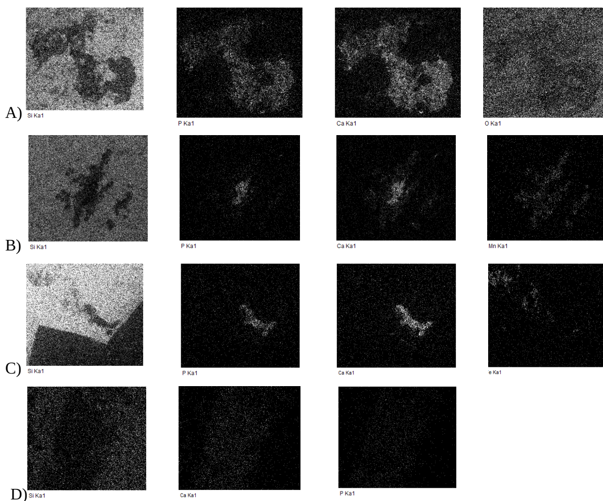
Figure 12: Element maps from SEM with EDX for the residue on the tools in figure 10. A) ) KLD-E6-5II-912; B) KLD59; C) KLD-E5-5-238; D) KLD-F6-5-741. Elements Si and O related to the tool, other residues are Mn (Manganese Oxide), Fe (Iron oxide) and P and Ca related to bone residue
