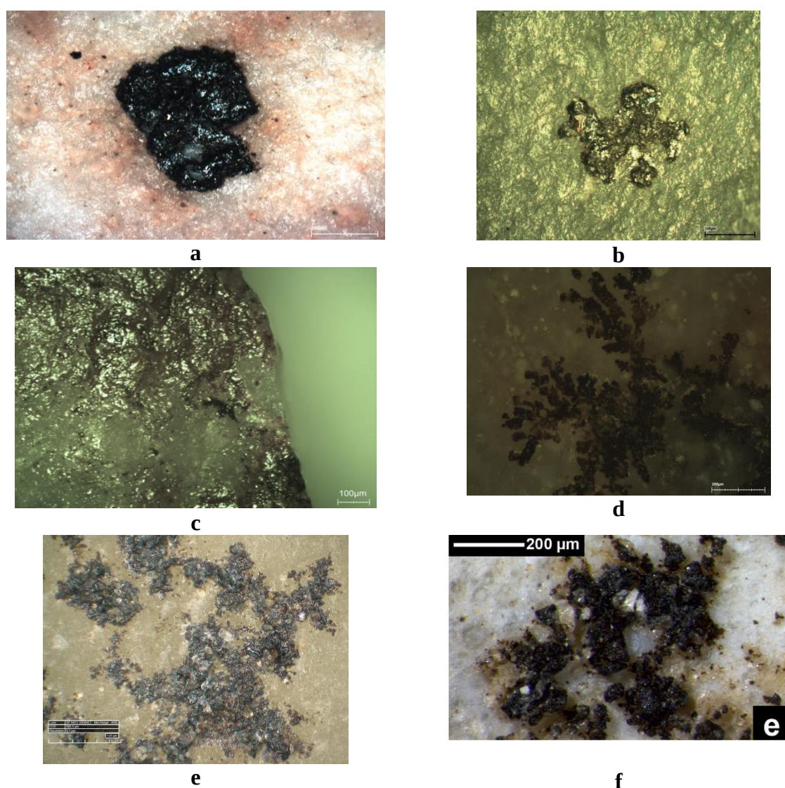
Figure 7: Type of black residue identified on the tools; a) black spot at 200x; b) in flower pattern (200x); c) greasy appearance 200x; d) like a lichen shape (100x); e) random shape (600x); f) black residue from Hummal Cave, Syria (Source Monnier et al. 2013)
