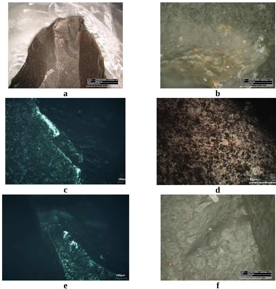
Figure 5.2: KLD-F6-7II-1145 ( Retouched Levallois point ) a) tip fracture at 35x; b) polish and striations at 700x green dot on the tool; c) location of the polish and fracture on the tip shown in yellow dot at 50x; d) same as (c) detail of the polish at 700x; e) polish on fracture at 50x; f) same as (e) detail of the polish at 700x
