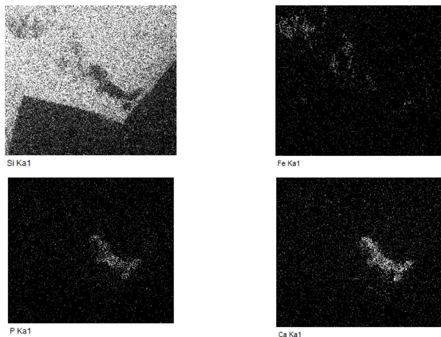
Figure 16: Showing element maps extracted from SEM with EDX for the residue of figure 13 (g-k). The elements are: Si (flint tool surface), Fe (for red residue), P and Ca (for bone residue)
