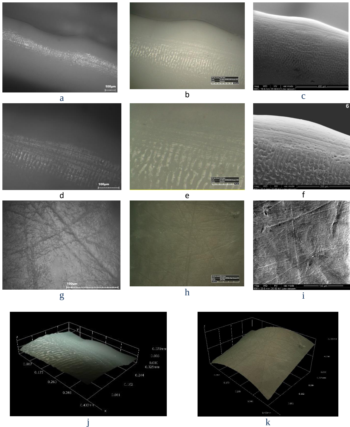
Figure 10: (a-f, j) RU01 (cutting wood, 10 minutes), (g-i, k) PE02 (disarticulating and defleshing 15 minutes); (a-c) location of the parallel striations to the edge with OLM at 100x, 3D DM at 400x, SEM 200x; (d-f) detail of the parallel striations to the edge with OLM at 200x, 3D DM at 1000x (high-range lens), SEM at 600x; (g-i) deep criss-cross striations with OLM at 500x, 3D DM at 700x, SEM at 600x; (j-k) 3D of the edge showing the location of the striations of the shell tool topography.
