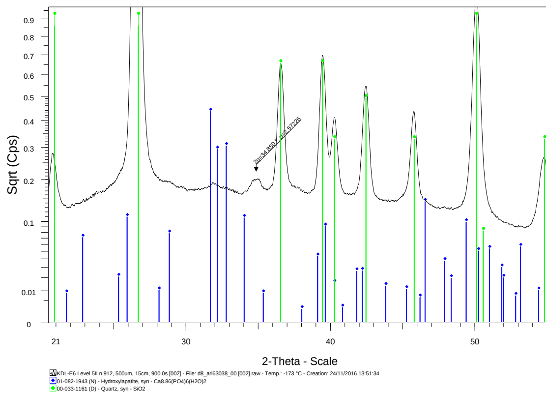
Figure 13: \mu XRD result showing the presence of Hydroxylapatite [ \text{Ca}_{8.86}(\text{PO}_4)_6(\text{H}_2\text{O})_2 ] represented by blue peaks and Green peaks represent quartz, syn-SiO 2
