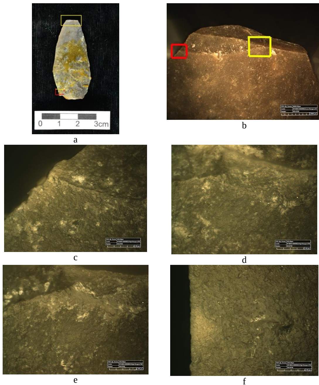
Figure 4.9: Zaragoza no 3 (arrowhead, 1 shot was performed) (a) showing the locations of the use-wear traces; b) detail view of the tip fracture (at 35x) showing the location of polished areas in (c-e) (at 700x; f) detail view of the polish on the tool marked in red box in Fig. (a) at 700x
