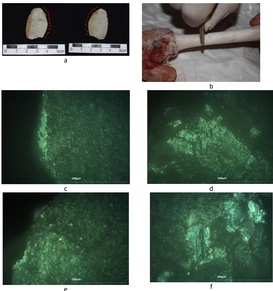
Figure 4.29: KF4-no 3 cutting bone (30 minutes) a) unused tool showing the working edge on the dorsal face (c-e) polish and edge rounding; f) ventral face polish and small deep striations parallel to the edge.
