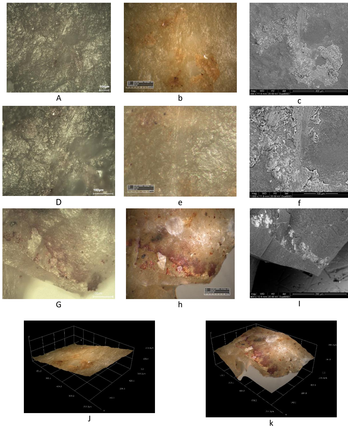
Figure 15: KLD-E6-5II-912 (Flake) (a-f ) showing the location of the amorphous colour bone residue and striation analyzed under SEM with EDX (at magnification 200x, 1000x), Hirox KH 8700 (at magnification 400x, 1000x), and Zeiss Axio scope A1 (at magnification 100x, 200x) and (j) 3D of the residue on the tool topography; (g-i) KLD-E5-5-238 (Twisted bladelet) showing red residue (Iron oxide) with bone residue with SEM with EDX (at mag 200x), Hirox 8700 (400x) and Zeiss Axio scope A1 (at 200x); (k) 3D of the residue location on tool topography
