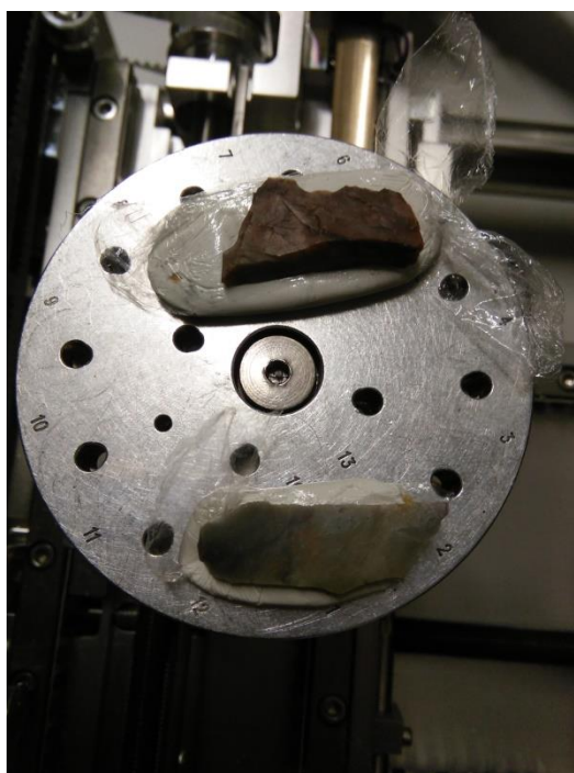
Figure 3.3. In the SEM chamber, archaeological tools placed on the moulding clay which is covered with cling plastic film
