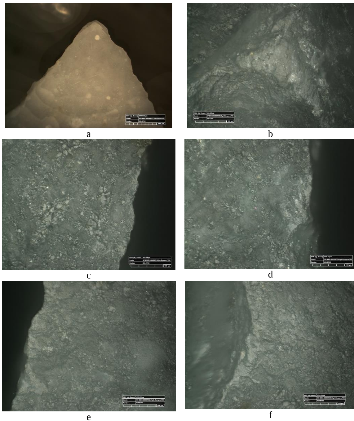
Figure 4.16: Ventral side of KHR6-no 1 (arrowhead, 10 shots were performed) (a) tip fracture at 35x; (b) polish with the striations; (c-f) hafting polish and edge rounding on the hafting area
