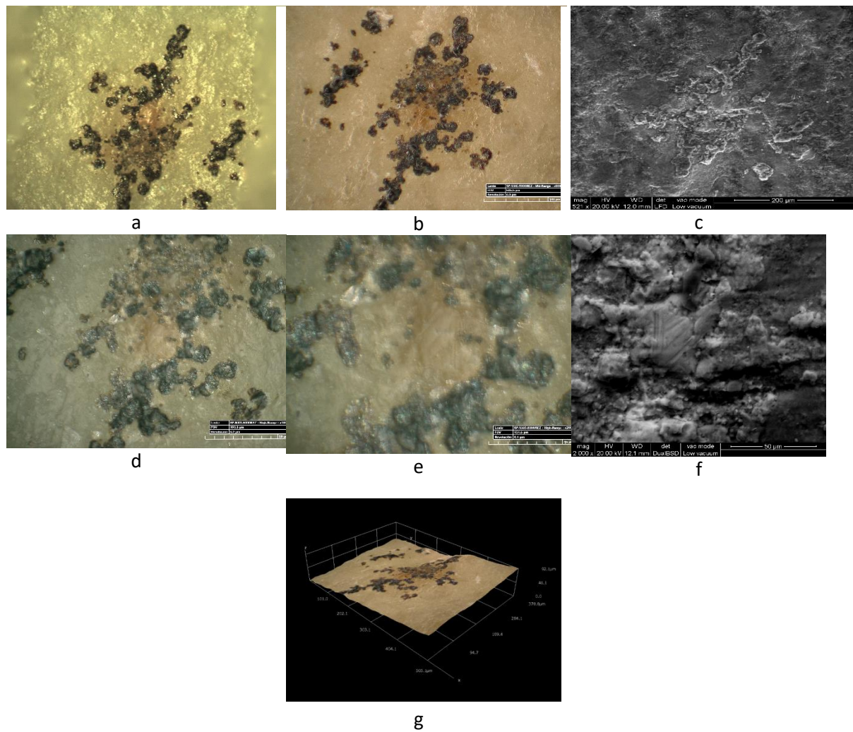
Figure 13: Kld 59 (Levallois Point) (a) Black residue with the pale brown residue underneath OLM at 100x magnification; (b and d-e) images with 3D DM showing the same residue at 600x (Mid-Range lens), 1000x and 2000x (high-range lens); (c-f) images with SEM showing the same residue as (a) at 521x and at 2000x residue with striations on them. 3D DM micrographs (a) is taken with a ring light and (d-e) are taken with coaxial light)
