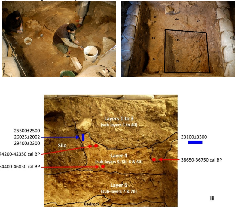
Figure 2: 1) Excavators with powder-free medical gloves to avoid any post-excavation contamination and finger flakes; 2) 3x3 m excavated trench and iii) Detailed stratigraphy of the excavation showing the layers and 3) the locations of the TL and C14 dating.
