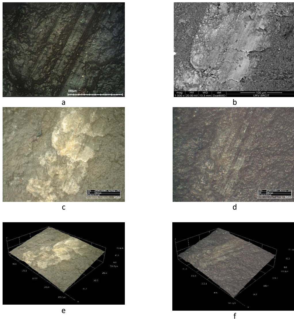
Figure 11: (a-f) KLD-F6-5-741 (Archaeological pointed bladelet; (a) deep striations under OLM at 500x; (b) detail of the striations showing bone residue adhere to it. Micrograph at 1000x; (c) same striations under 3D DM at with high-range lens at 700x; (d) same striations under 3D DM with Mid-Range lens at 600x with coaxial light.
