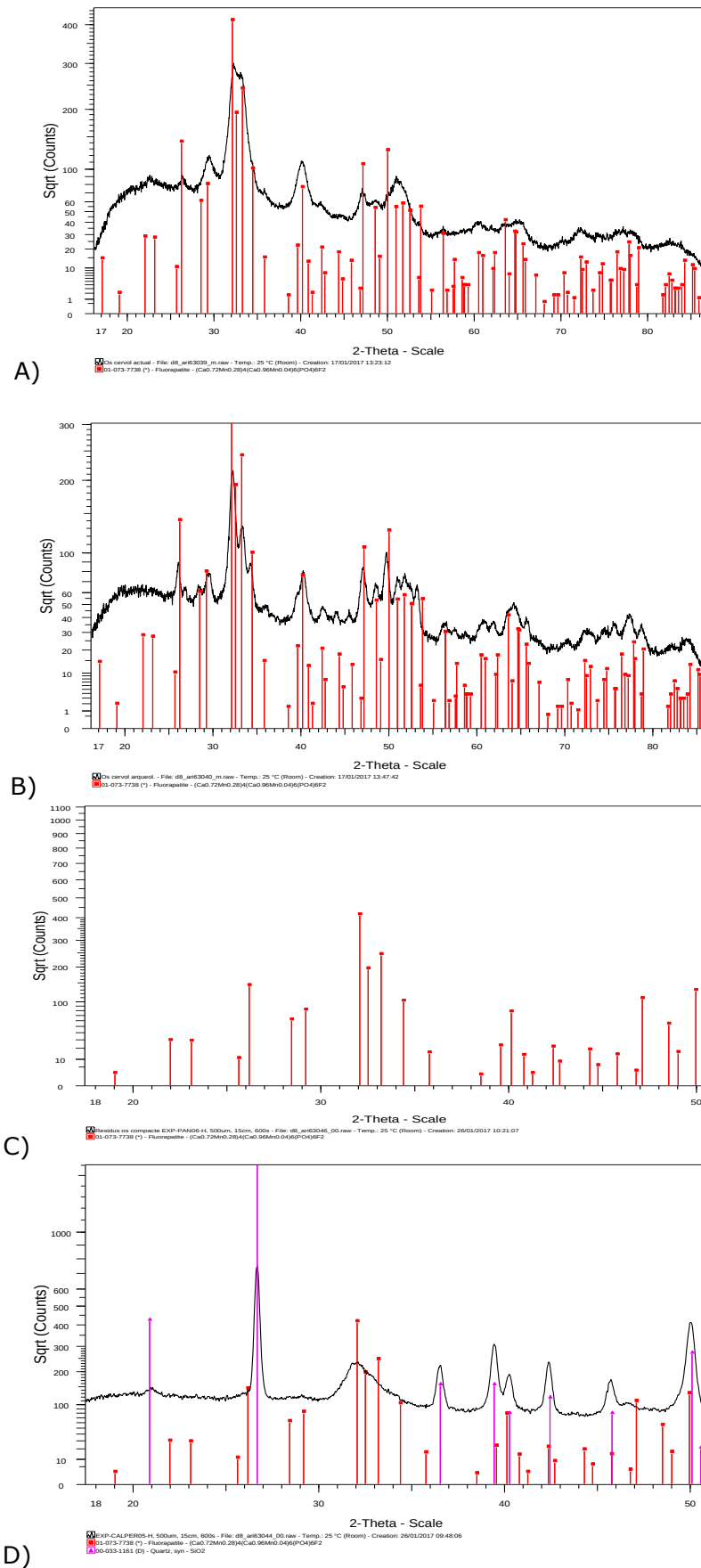
Figure 15: \mu XRD spectra a) powder of bone and b) experimental piece with bone residue on the edge, c) and d) Pink peak represent Fluorapatite and red peaks represent \text{SiO}_2
