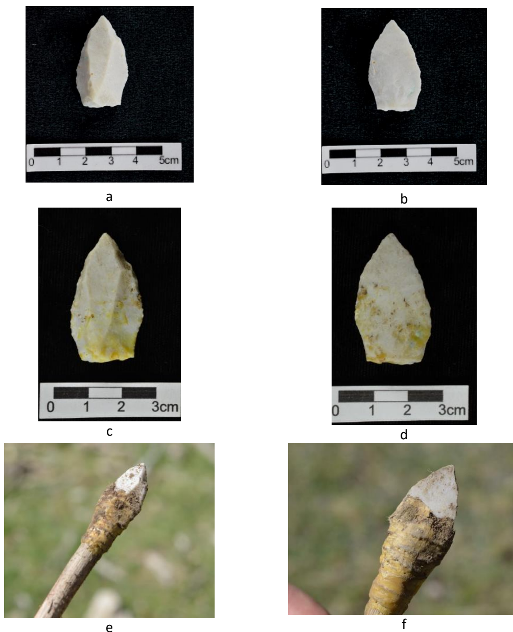
Figure 4.17: KHR4 no 4 (arrowhead, 10 shots were performed) (a-b) dorsal and ventral of the unused tool; (c-d) showing the distribution of the adhesive on the tool surface; (e-f) after pierced in the ground tool covered with the soil on it.
