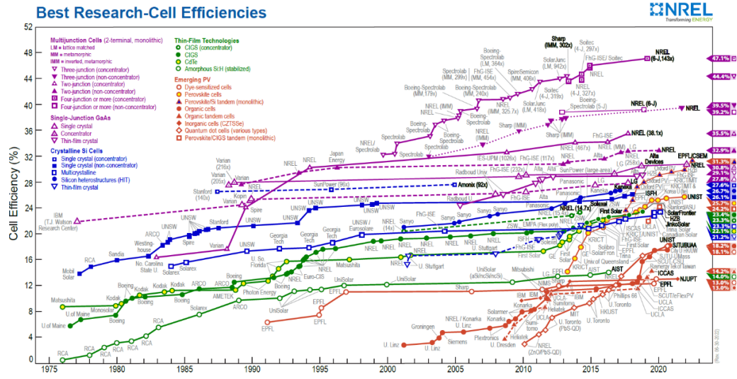
Figure 1.2 Chart of the recent photovoltaics efficiencies that summarized by NREL 27
