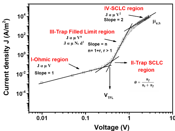
Figure 2.10 Typical SCLC behavior for organic semiconductors.
