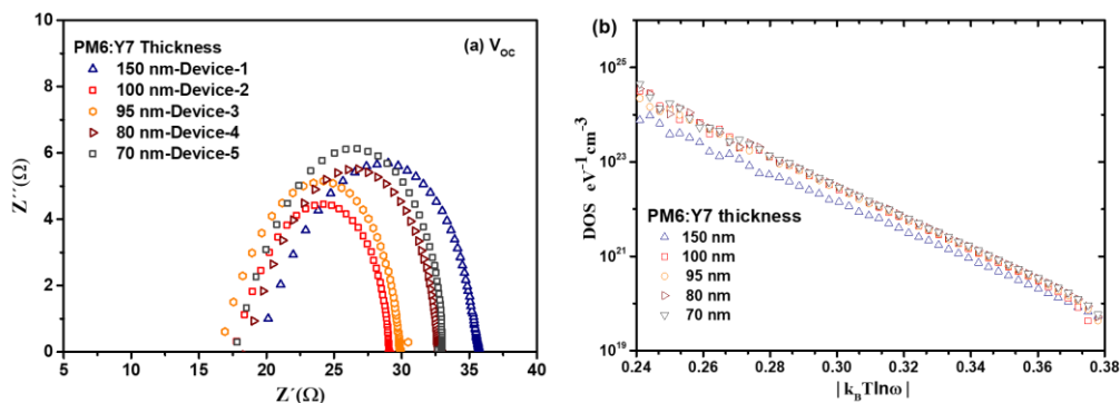
Figure 6.4 (a) Cole-Cole plots, (b) DOS as function of |k_B T \ln \omega| at V_{OC} under AM1.5 G illumination, of different thicknesses of the PM6:Y7 photoactive layer-based NF-OPVs.
