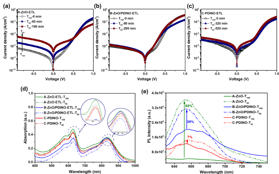
Figure 5.6 J-V characteristic curves of the T 100 fresh and T 90 , T 80 photo-degraded iNF-OSCs at dark of (a) A-ZnO, (b) B-ZnO/PDINO, and (c) C-PDINO based devices, (d) UV-vis optical characteristics of the T 100 and T 80 photo-aged PM6:Y7 blend films over different ETLs, (e) Photoluminescence spectra of the T 100 and T 80 photo-aged PM6:Y7 blend films over different ETLs
