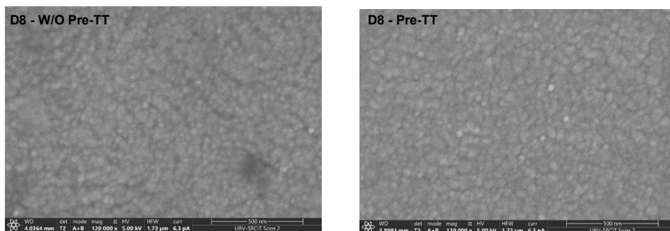
Figure 6.21 Field emission scanning electron microscope images of the D8 pristine and Pre-TT PEDOT:PSS/PM6:Y7 based films.
