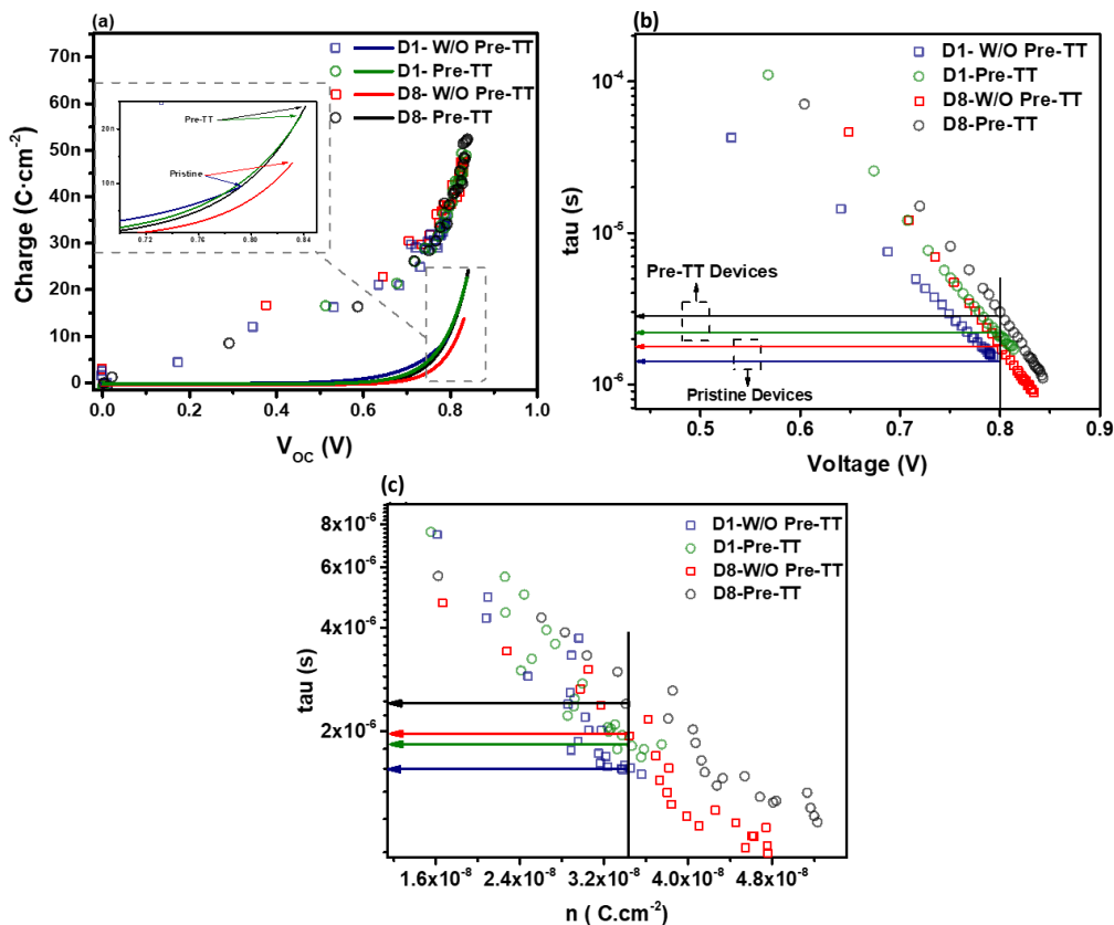
Figure 6.12 (a) Charge measured at different light biases for the pristine and Pre-TT devices. The symbols correspond to both geometrical capacitance and chemical capacitance. The solid lines at the bottom represent only the exponential part: y=Be^{Cx} (chemical capacitance) after subtraction of the geometrical capacitance, (b) TPV versus voltage of the pristine and Pre-TT NF-OPVs devices, (c) charge measured by CE versus the carrier lifetime obtained via TPV for the pristine and Pre-TT devices.
