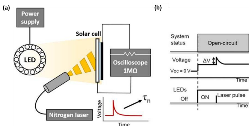
Figure 2.13 (a) Schematic illustration of the transient photovoltage setup and (b) the demonstrated corresponding signals that can be monitored at the oscilloscope 175 .
