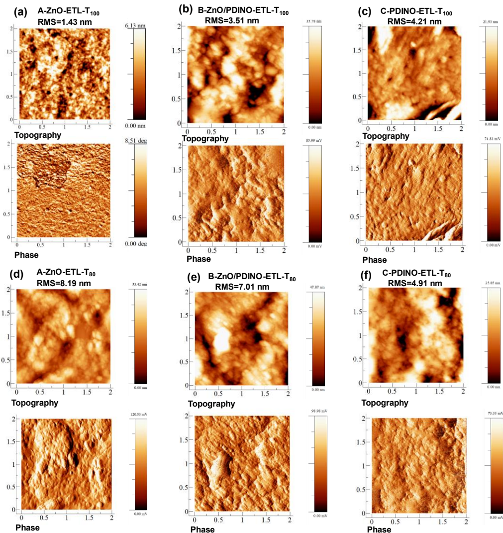
Figure 5.14 AFM topography and phase images of the PM6:Y7 blend films over different ETLs of T 100 (a) A-ZnO, (b) B-ZnO/PDINO, (c) C-PDINO based films and the T 80 photo-degraded (d) A-ZnO, (e) B-ZnO/PDINO, (f) C-PDINO based films.
