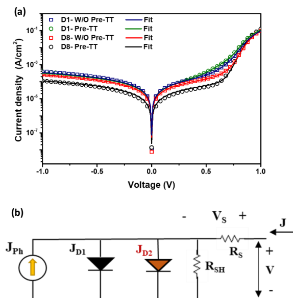
Figure 6.10 (a) J-V characteristic curves of the pristine and the Pre-TT NF-OPVs of D1 and D8 at dark condition (symbols for experimental data and the lines for the fitting). (b) Equivalent electrical circuit used to fit the experimental dark current-voltage measurements ( J_{ph} = 0 ) of the NF-OPVs corresponding devices.
