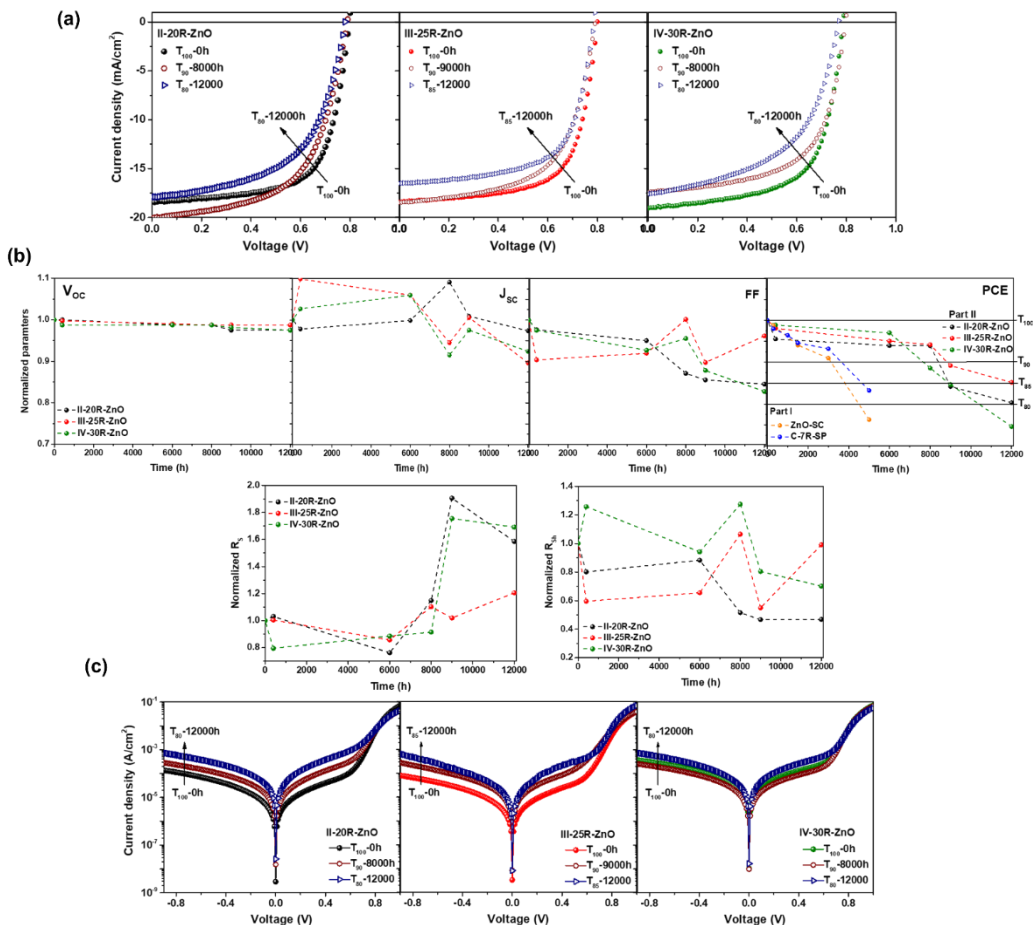
Figure 3.16 (a) Current density- voltage ( J-V ) characteristic curves under AM 1.5 G illumination, (b) the normalized performance parameters, (c) J-V characteristic curves at dark of the degraded iF-OPVs with respect to the aging time (12000 h)- devices stability study
