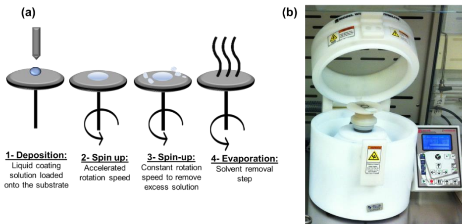
Figure 2.3 (a) The four stages of the spin coating procedures, (b) the lab spin coater machine used in this thesis.
