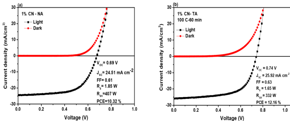
Figure A.7 Current density-voltage (J-V) characteristic curves under Illumination (AM 1.5 G) of the binary iNF-OPVs treated with 1 % CN additives (a) non-annealed (NA) and (b) thermally annealed (TA) at 100 °C for 60 min.
