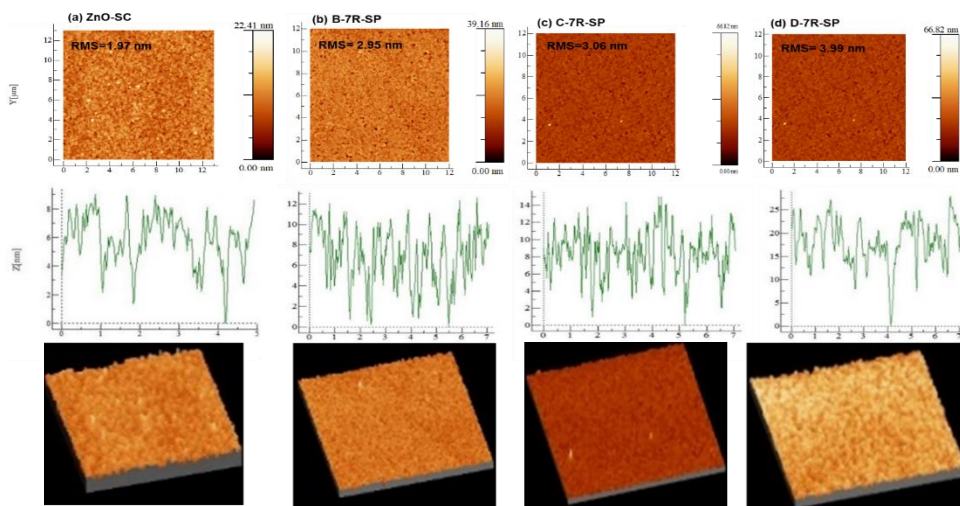
Figure 3.4 AFM topographical images of the ZnO films deposited by SC (a) and 7R-SP devices of B (b), C (c) and D (d) concentrations.
