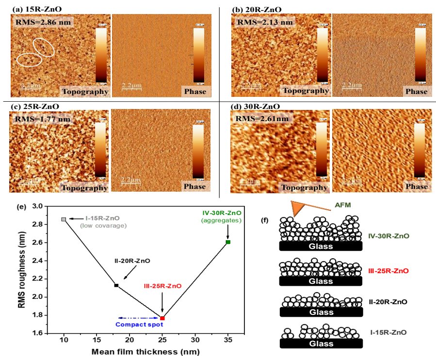
Figure 3.14 AFM topographic and phase images of the ZnO film with (a) 15R (Thickness=10 nm), (b) 20R (Thickness=18 nm), (c) 25R (Thickness=25 nm), and (d) 30R (Thickness=35 nm). (e) RMS surface roughness of ZnO films as a function of film thickness. (f) Schematics simplifying the evaluated ZnO surface morphology measured by the AFM tip.
