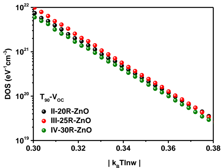
Figure A.6 DOS as function of |k_B T \ln \omega| at V OC under AM 1.5G illumination of the T 90 degraded iF-OPVs.
