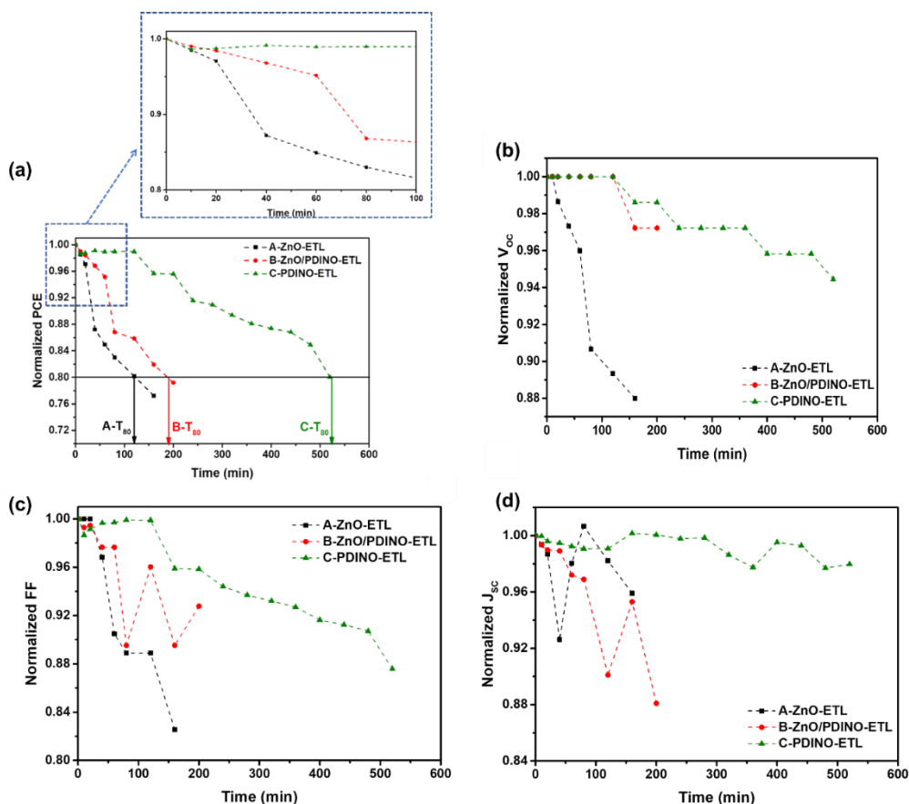
Figure 5.5 Normalized performance parameters of the iNF-OSCs (a) PCE, (b) V_{oc} , (c) FF, and (d) J_{sc} of the iNF-OSCs over photo-aging time.
