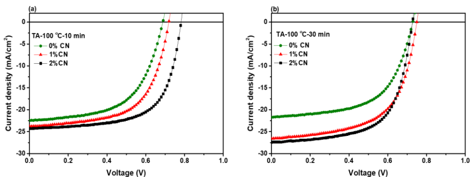
Figure A.8 Current density-voltage (J-V) characteristic curves under Illumination (AM 1.5 G) of the binary iNF-OPVs treated with different percentage of CN additives and thermally annealed at 100 °C for (a) for 10 min and (b) 30 min.
