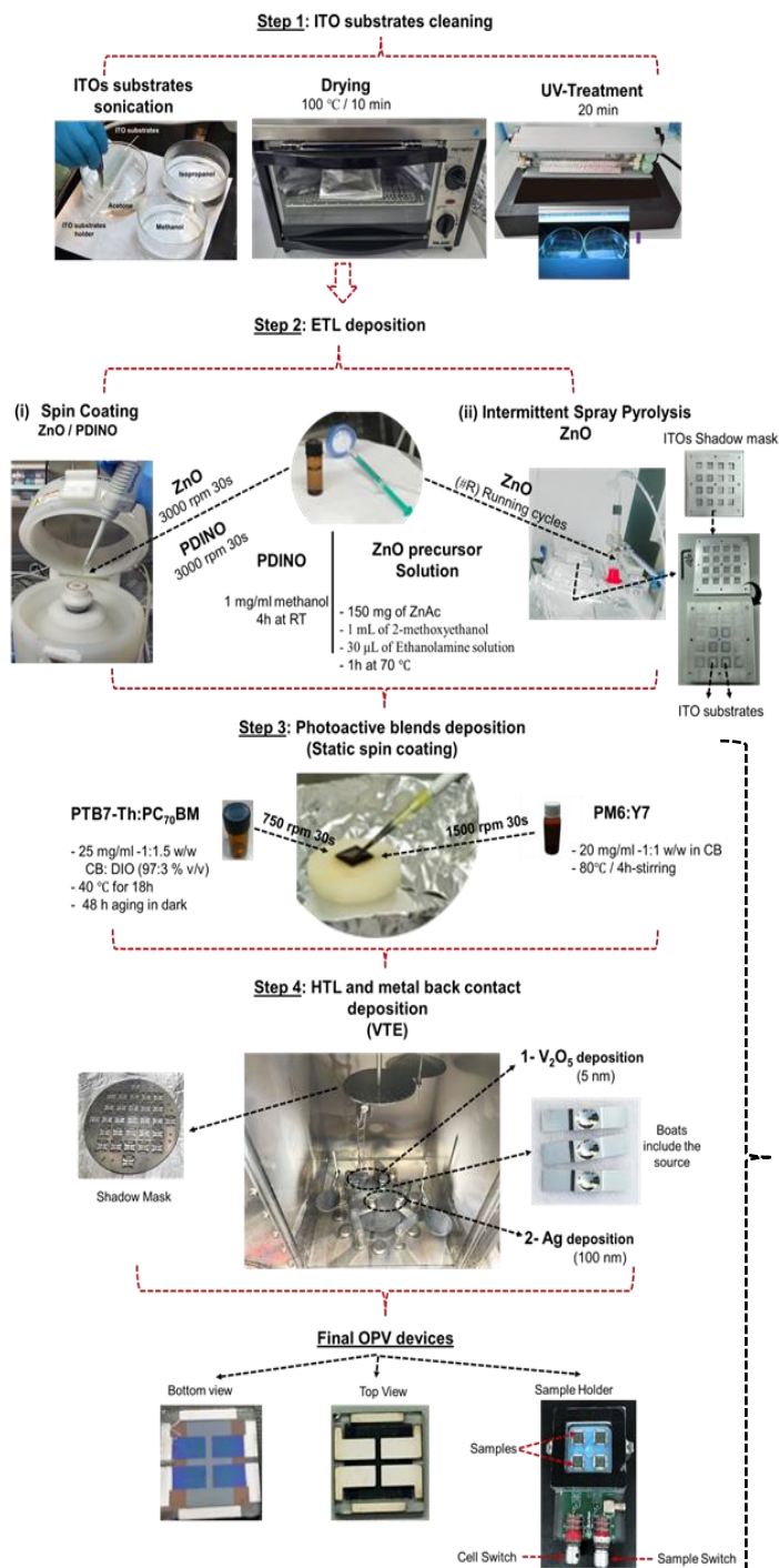
Figure 2.8 Schematic diagram illustration for the fabrication procedures of the inverted structure OPV devices in this thesis.
