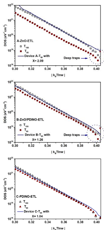
Figure 5.10 DOS as function of |k_B T \ln \omega| at V_{OC} under AM 1.5G illumination of the T_{100} and T_{80} photo-aged iNF-OPVs over times (blue line with shifting value of X), (a) A-ZnO, (b) B-ZnO/PDINO, and (c) C-PDINO based devices.
