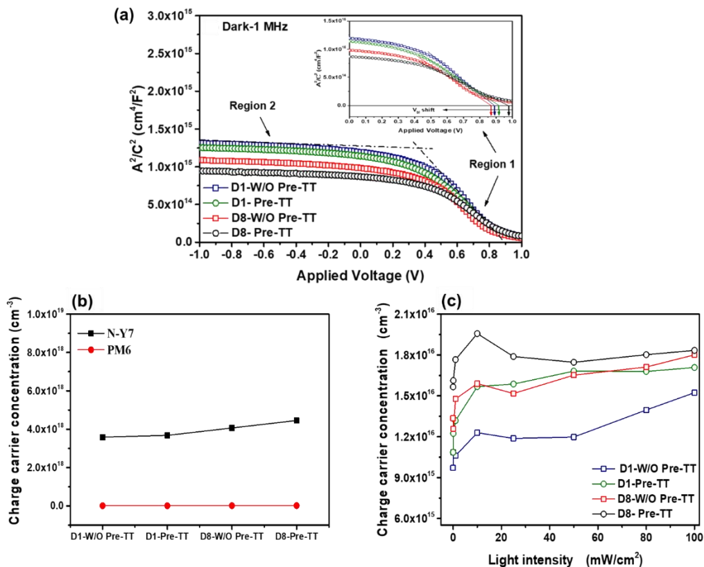
Figure 6.19 (a) Mott Schottky plot at dark at 1 MHz of the pristine and Pre-TT D1 and D8 NF-OPVs. (b) Charge carrier concentration in region 1 (PM6-donor polymer) and region 2 (Y7-acceptor polymer) plot for the fabricated pristine and Pre-TT D1 and D8 devices, this data extracted from the CV measurements taken at 1 MHz under dark (in Figure 6.19a) applying equation 6.6 then equation 6.7. (c) Charge carrier concentration in region 1 (PM6-donor polymer) plot vs the illumination intensities for the devices. The values extracted from the CV measurements were taken at 1 MHz for each P_{\text{light}} condition, then applied equation 6.6.
