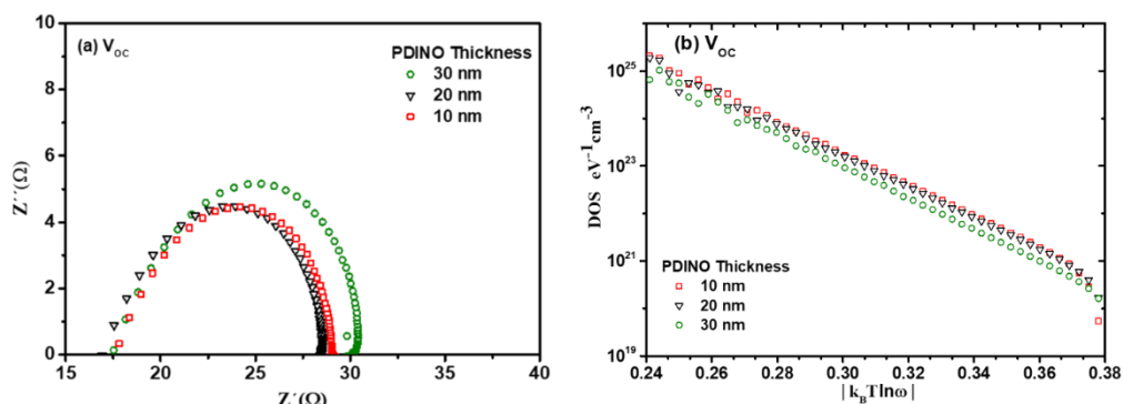
Figure 6.8 (a) Cole-Cole plots, (b) DOS as function of |k_B T \ln \omega| at V_{OC} under AM1.5 G illumination of different PDINO thicknesses-based NF-OPVs.
