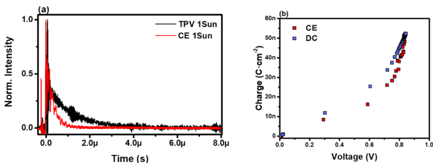
Figure A.16 (a) Comparison of CE and TPV decays at 1 Sun illumination and (b) charge vs voltage obtained by using CE and the combination of TPV/TPC (DC) techniques for D8-Pre-TT devices.
