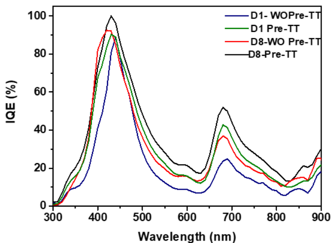
Figure A.14 IQE spectral response of the pristine and Pre-TT D1 and D8 based devices.
