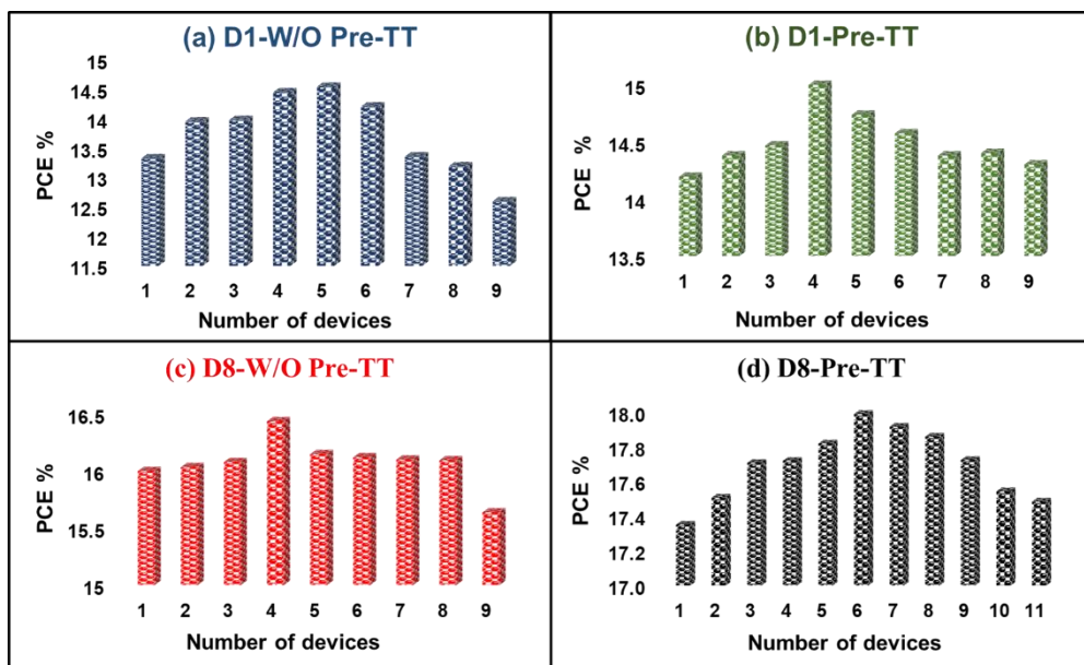
Figure A.13 The PCE % statistics diagrams for the fabricated (a) D1-W/O Pre-TT, (b) D1- Pre-TT, (c) D8-W/O Pre-TT, and (d) D8-Pre-TT NF-OPVs devices.
