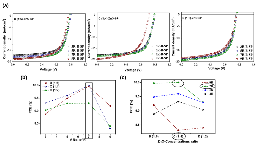
Figure 3.3 (a) J-V characteristic curves of the iF-OPVs devices fabricated by intermittent SP technique at running cycles of 3R, 5R, 7R, and 9R for each ZnO precursor solution concentration under illumination, (b) PCE vs R (c) PCE of the iF-OPVs vs B, C and D ZnO precursor solution concentrations.
