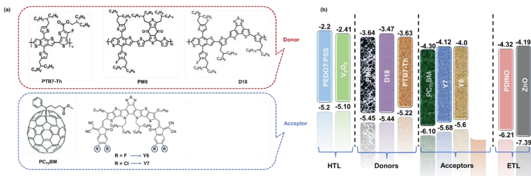
Figure 2.1 (a) The molecular structures of the conjugated donor polymers and small molecule fullerene, nonfullerene acceptors studied in this thesis, (b) The energy levels of the photoactive, ETLs and HTLs materials studied in this thesis.
