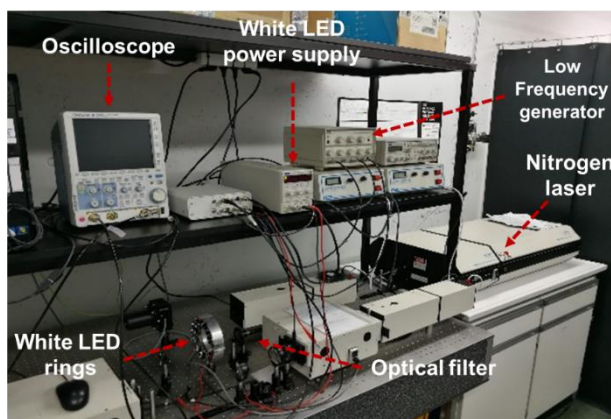
Figure 2.16 The experimental setup used in this thesis for charge extraction and transient photovoltage/photocurrent measurements in ICIQ.
