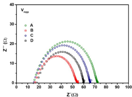
Figure A.9 Nyquist Plots of the pristine and treated iNF-OPVs devices under AM 1.5G illumination and an oscillation amplitude of 50 mV at V_{MPP} bias voltage.
