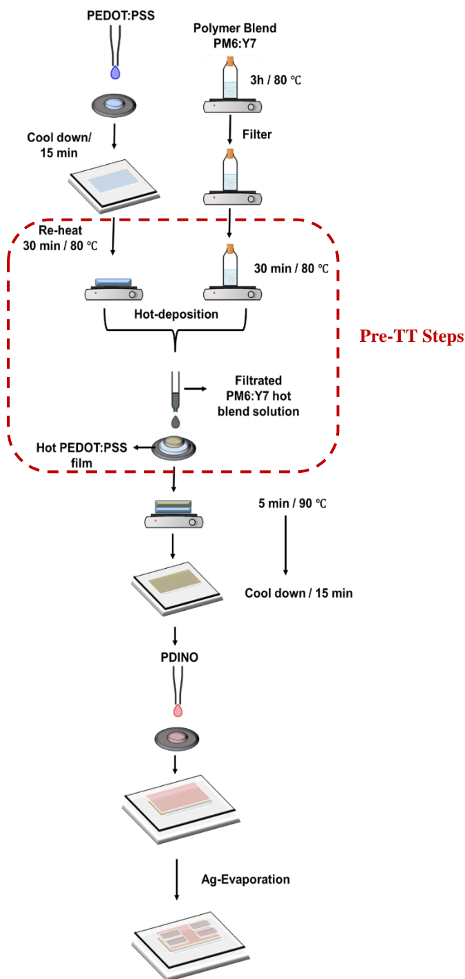
Figure 6.2 Scheme of the proposed Pre-Thermal Treatment (Pre-TT) Approach procedures for the Pre-TT NF-OPVs based devices.
