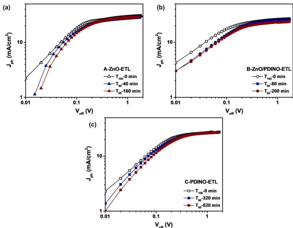
Figure 5.8 J_{ph} versus V_{eff} characteristics of the T_{100} , T_{90} and T_{80} (a) A-ZnO, (b) B-ZnO/PDINO, and (c) C-PDINO based devices over photo-aging time.
