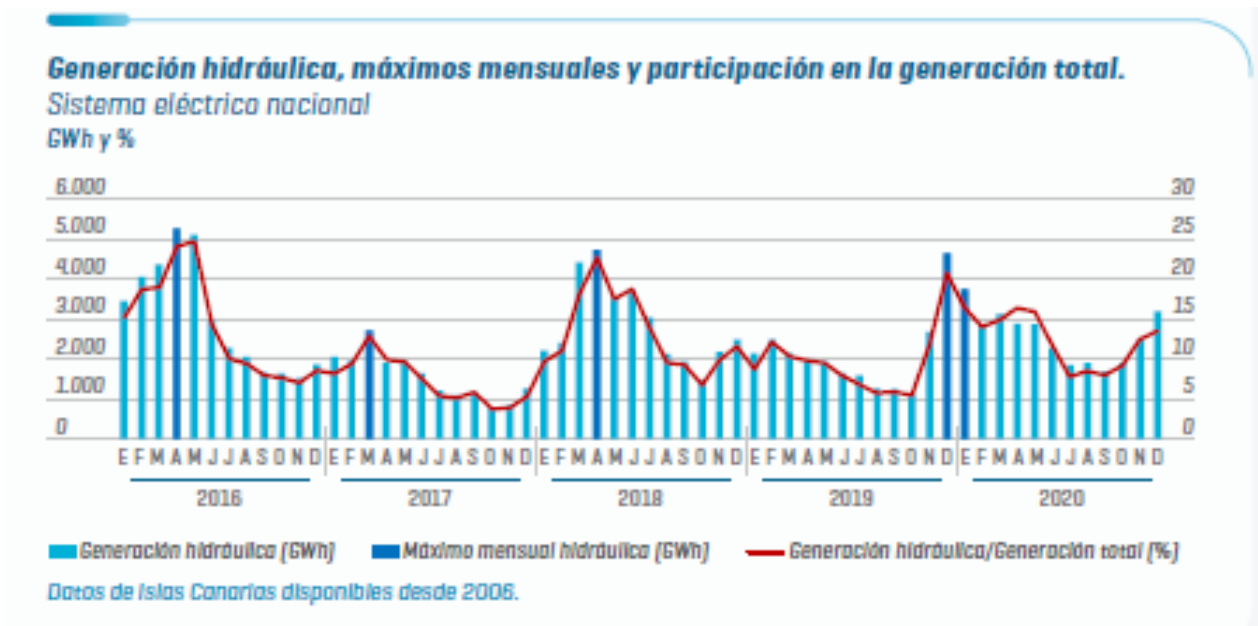
Figure 29 Monthly percentage of hydroelectric generation in Spain [18]
