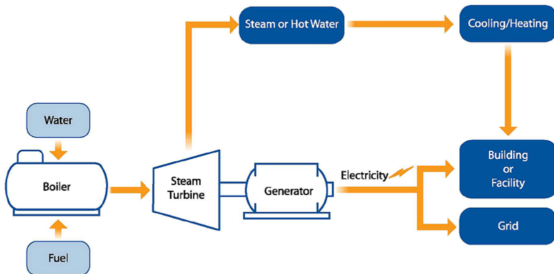
Figure 3 Scheme of a Combined Heat and Power plant [5]
