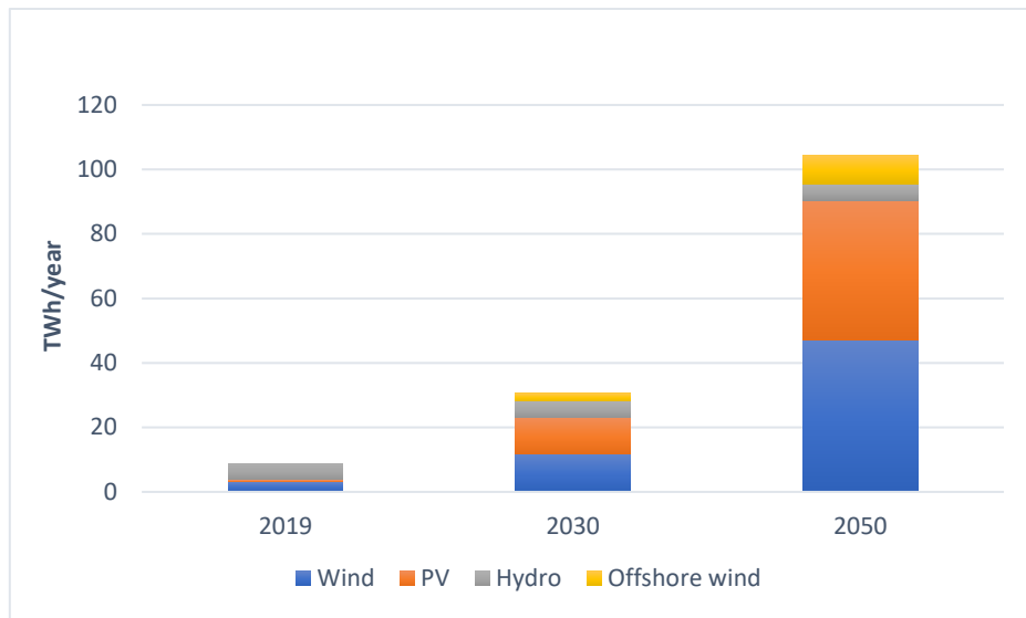
Figure 33 Renewable electricity production in different scenario
