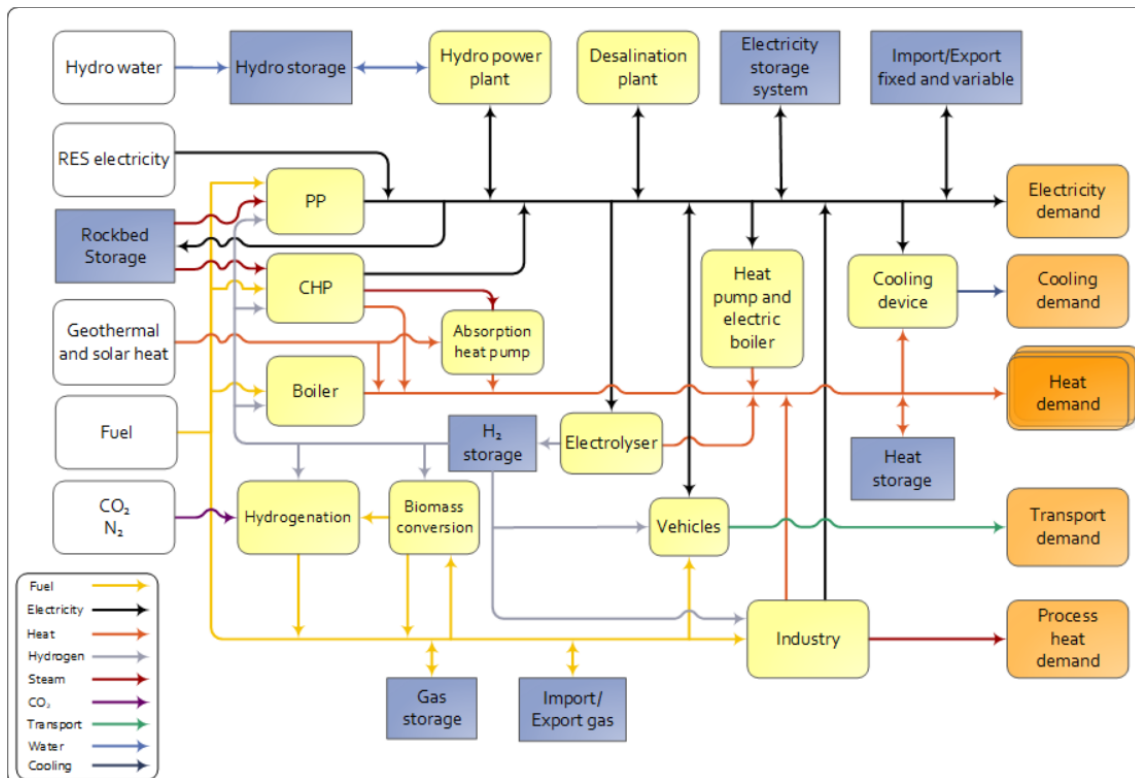
Figure 6 Scheme of a smart energy system from EnergyPlan [1]
