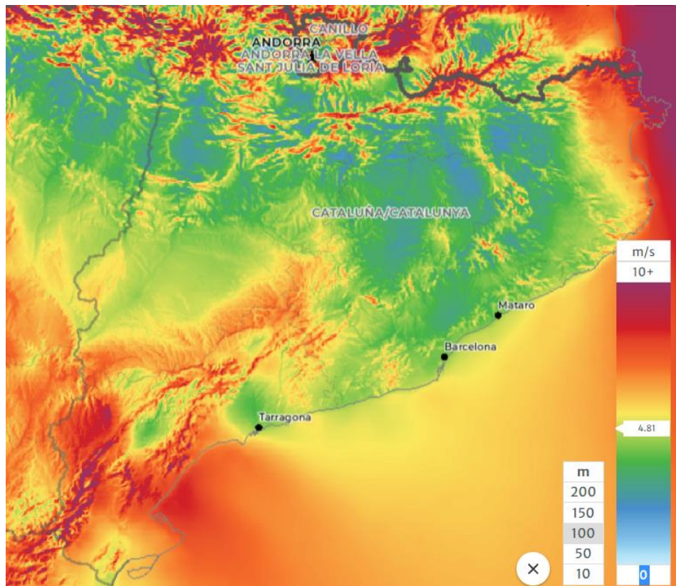
Figure 22 Wind speed in Catalonia [14]
