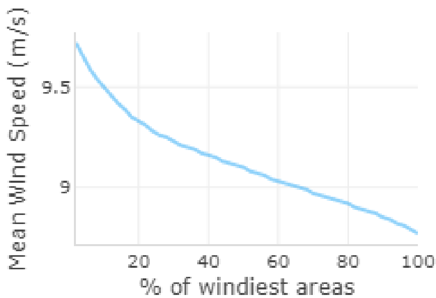
Figure 23 Duration curve of wind speed [14]
