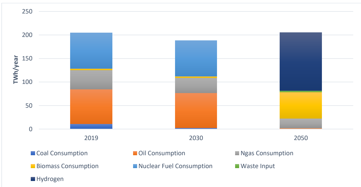
Figure 34 Fuel consumption of different scenarios
