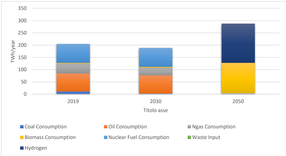
Figure 35 Fuel consumption required to fully replace natural gas
