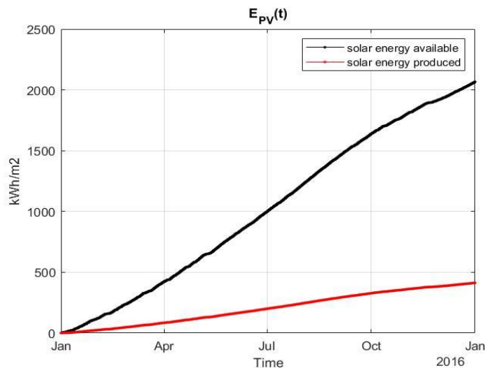
Figure 27 Comparison of energy available and electricity produced
