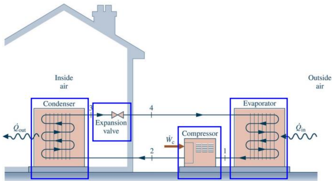
Figure 4 Scheme of a heat pump installed in building [6]
