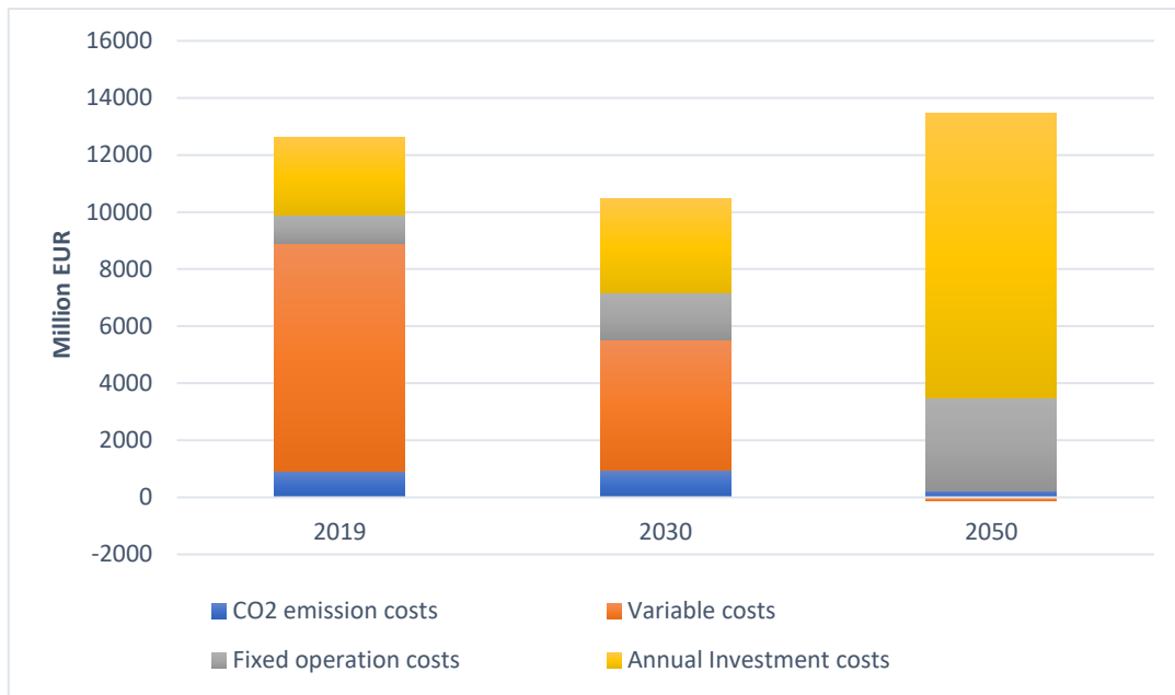
Figure 37 Annual costs of different scenarios
