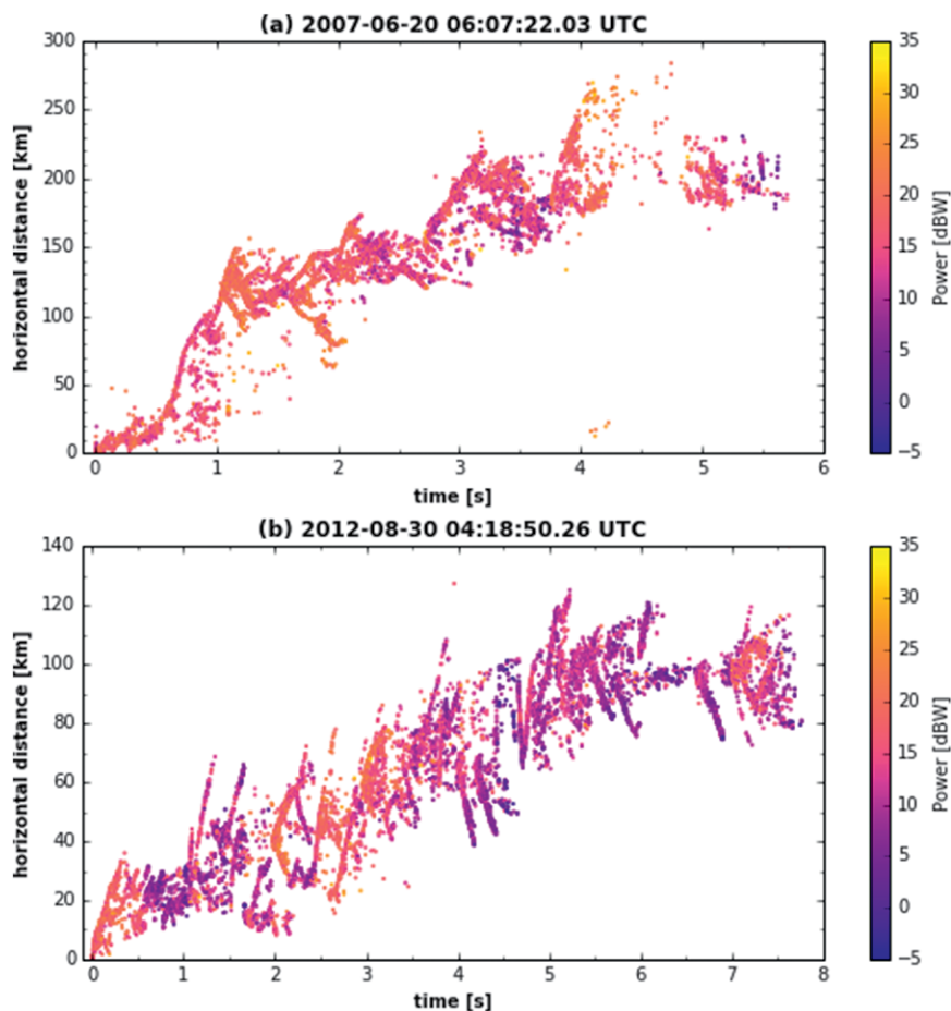
FIG. 4. Time vs horizontal distance as a function of power (dBW) showing the lightning events of (a) 0607:22 UTC 20 Jun 2007 in Oklahoma and (b) 0418:50 UTC 30 Aug 2012 in southern France. For interpretation of the time-vs-distance plot, see van der Velde and Montanyà (2013).
