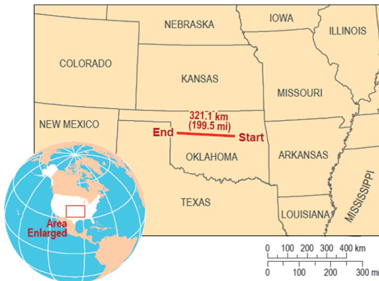
FIG. 1. Linear representation of the Oklahoma flash event for 0607:22 UTC 20 Jun 2007 using the maximum great circle distance method described in the text; the WMO-evaluated “longest distance lightning flash” event.
