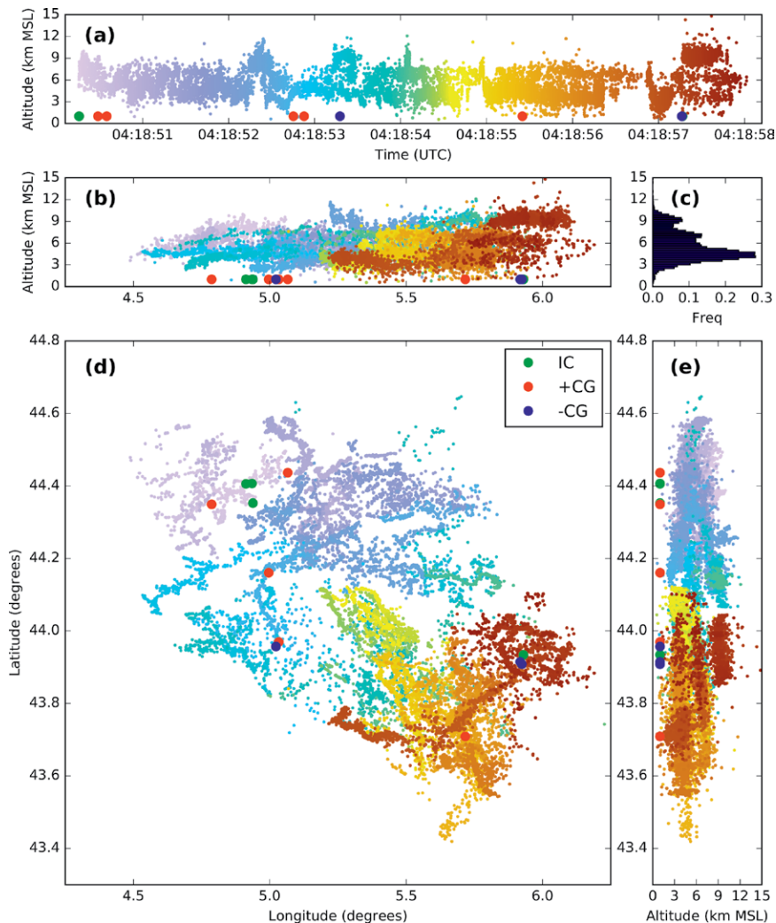
FIG. 8. Characteristics of the southern French flash event at 0418:50 UTC 30 Aug 2012. (a) Time–height (km MSL) evolution with color variations indicating time intervals, (b) longitude (°)–altitude (km MSL) plot, (c) altitude (km MSL)–frequency diagram, (d) latitude–longitude plot time-sequenced flash event, and (e) altitude (km, MSL)–latitude (°) plot. Also shown on most panels are locations and times of EUCLID-detected ICs, positive CGs, and negative CGs.
