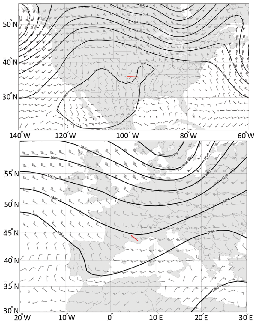
FIG. 5. Twentieth Century Reanalysis (v2) of the 500-hPa height (m) over (top) North America at 0600 UTC 20 Jun 2007 and (bottom) Europe at 0600 UTC 30 Aug 2012.
