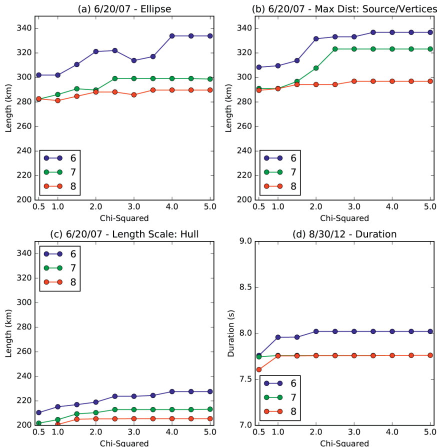
FIG. 6. Computation of the flash length using the four different methods discussed in the text for a variety of stations and \chi^2 values for the Oklahoma flash event at 0607:22 UTC 20 Jun 2007. Colors are used for the minimum number of stations (blue, 6; green, 7; red, 8). (a) Ellipse method. (b) Maximum distance between two individual sources or maximum distance between convex hull vertices, which are mathematically equivalent. (c) Characteristic length scale of the convex hull. (d) Comparison of flash durations for the France flash event at 0418:50 UTC 30 Aug 2012, for a variety of station numbers and \chi^2 thresholds. The seven- and eight-station curves largely overlap.
