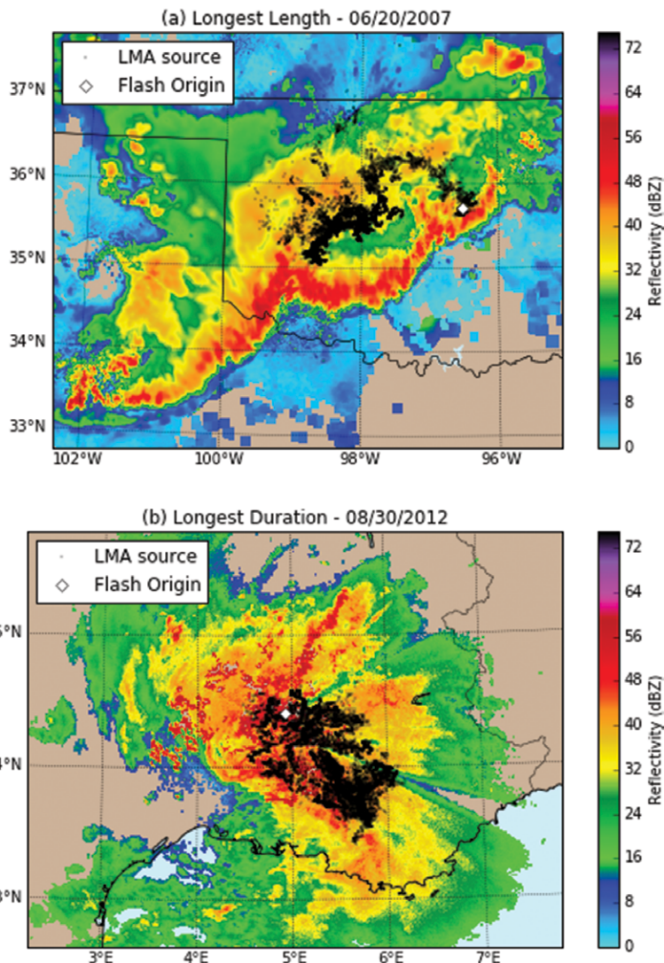
FIG. 2. (a) Mosaic radar reflectivity at 1 km MSL, valid at 0603 UTC 20 Jun 2007. Also shown is a plan projection of the VHF sources encompassing the longest-length flash, which occurred around 0607:22 UTC on this day. See Lang et al. (2010) for more details about this multiradar mosaic product. Flash origin is set as the median of the first 10 sources. (b) Reflectivity from the Aramis (Bollène) radar at 0.8° elevation angle, valid at 0415 UTC 30 Aug 2012. Ground clutter has not been edited from these data. Also shown is a plan projection of the VHF sources encompassing the longest-duration flash, which occurred around 0418:50 UTC on this day. Flash origin is set as the median of the first 10 sources.
