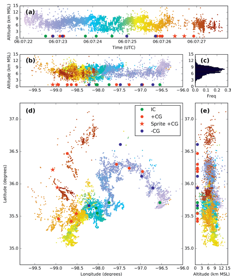
FIG. 3. Characteristics of the Oklahoma flash event for 0607:22 UTC 20 Jun 2007. (a) Time–height (km MSL) evolution with color variations indicating time intervals, (b) longitude (°)–altitude (km MSL) plot, (c) altitude (km MSL)–frequency diagram, (d) latitude–longitude plot time-sequenced flash event, and (e) altitude (km, MSL)–latitude (°) plot. Also shown on most panels are locations and times of NLDN-detected ICs, positive CGs, and negative CGs.
