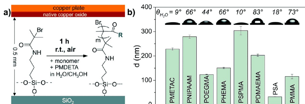
Figure 13. (a) Reaction scheme for the surface-initiated polymerization using a surface-modified silicon wafer piece bearing a standard initiator, a facing copper plate at a distance of 0.5 mm, and a solution of the monomer with the ligand (PMDETA) in water/methanol. (b) Polymer brush layer thickness, d , as determined by ellipsometry and water contact angles for the polymer brushes after SI-CuCRP for 1 h at ambient conditions (room temperature, handling in air). Reproduced with permission from ref 249 under a Creative Commons Attribution 3.0 Unported License ( https://creativecommons.org/licenses/by/3.0/ ). Published by The Royal Society of Chemistry.
