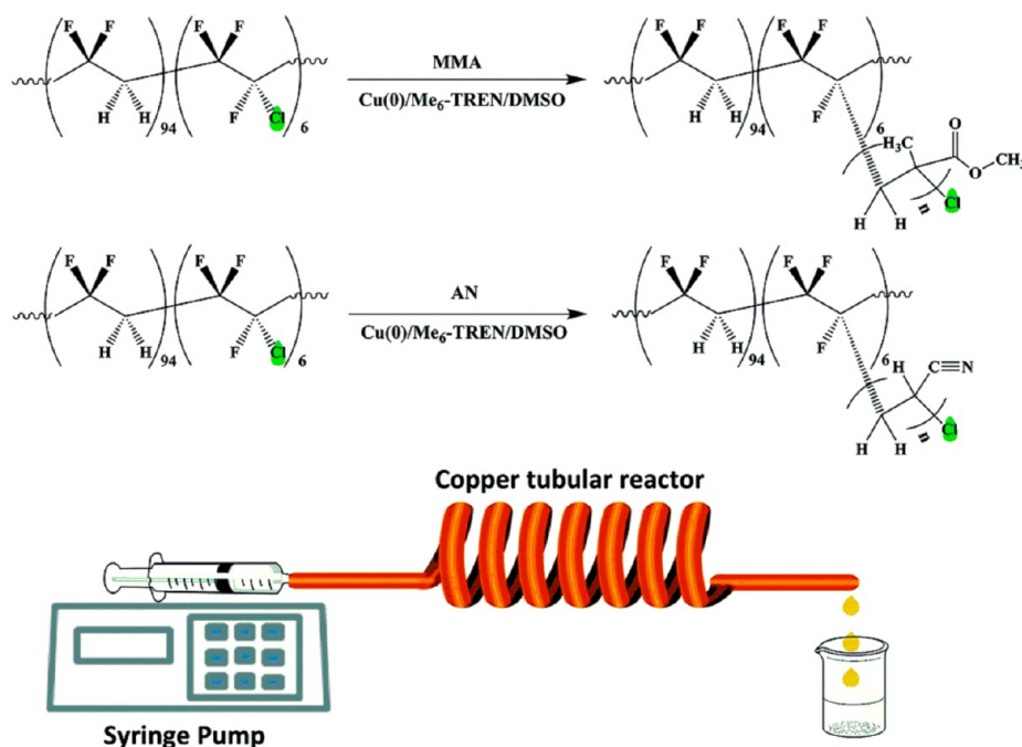
Figure 5. SET-LRP of MMA and AN initiated with P(VDF-co-CTFE) and a schematic diagram of the copper tubular reactor. Reproduced from ref 104, with permission of The Royal Society of Chemistry. http://dx.doi.org/10.1039/c5py01728a .
