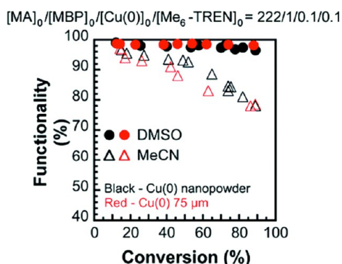
Figure 3. Evolution of bromine chain-end functionality with conversion in solvents mediating different degrees of disproportionation. Reaction conditions: MA = 1 mL, solvent = 0.5 mL, [MA]_0/[MBP]_0/[Cu(0)]_0/[Me_6-TREN]_0 = 222:1:0.1:0.1 , 25 °C, Cu(0) 75 \mu\text{m} or Cu(0) nanopowder. Reproduced with permission from ref 168. Copyright 2012 American Chemical Society.
