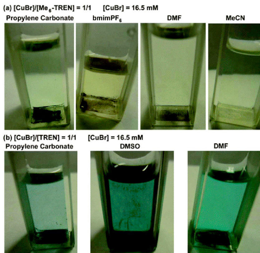
Figure 2. Visual observation of Cu(0) nanoparticles and CuBr 2 generated from the disproportionation of CuBr in polar aprotic solvents in the presence of Me 6 -TREN (a) and TREN (b). Conditions: solvent = 1.8 mL; [CuBr]/[N-ligand] = 1:1. Pictures were taken 10 min after mixing the reagents. Reproduced from ref 14, with permission of The Royal Society of Chemistry. http://dx.doi.org/10.1039/C2PY21084C .
