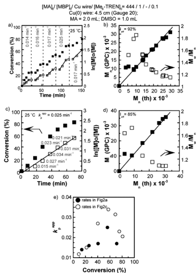
Figure 1. Kinetic plots of SET-LRP of MA initiated by methyl 2-bromopropionate (MBP) in DMSO at 25 °C using 4.5 cm of 20 gauge Cu(0) wire as catalyst (a and b) with four time exposures to air flow during the middle of reaction and (c and d) without air exposure; (e) plot of rate constants obtained from (a and c) versus conversion of monomers. Reaction conditions: [MA]_0/[MBP]_0/[Me_6-TREN]_0 = 444:1:0.1 , [MA]_0 = 7.4 mol/L, MA = 1.0 mL, DMSO = 0.5 mL. Reproduced from ref 120, with permission from John Wiley and Sons. Copyright 2010 Wiley Periodicals, Inc.
