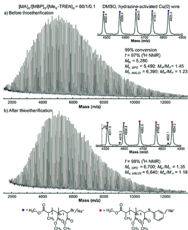
Figure 4. MALDI-TOF spectra of monofunctional PMA obtained at 99% conversion ( M_n = 5490 , M_w/M_n = 1.45 ) (a) before and (b) after nucleophilic displacement of the bromine chain end with thiophenol. Polymerization conditions at 25 °C: MA = 2 mL, DMSO = 1 mL, [MA]_0/[MBP]_0/[Me_6-TREN]_0 = 60:1:0.1 , hydrazine-activated Cu(0) wire = 0.5 cm of 20 gauge wire. Reproduced with permission from ref 168. Copyright 2012 American Chemical Society.
