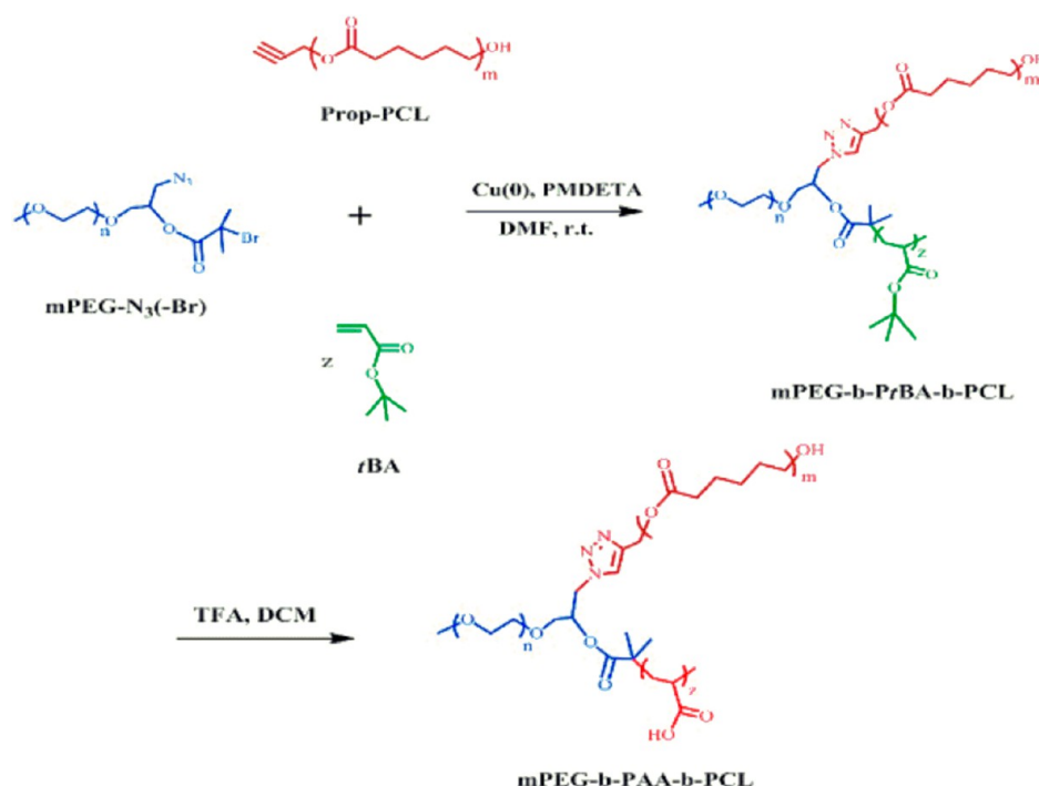
Figure 10. Synthesis of ABC miktoarm star terpolymers in one-pot combining click chemistry and SET-LRP. Reproduced from ref 206, Copyright (2015), with permission from Elsevier.
