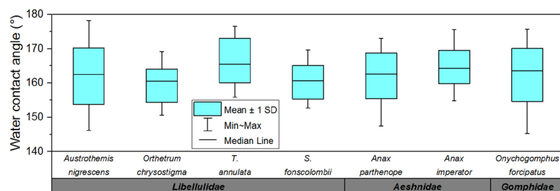
Figure 2. Wettability of the wing surface of seven species of dragonfly from three families. WCAs were measured using a sessile drop at 17 points across the wing surface. Figure created using OriginPro 2015 (OriginLab Corporation, Northampton, MA).
