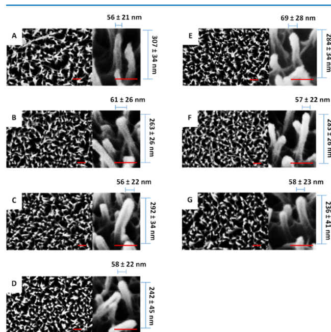
Figure 4. Top-view (left) and tilted (right) images of nanopillar arrangements on the wing epicuticle of seven species of dragonfly from three families. (A) Austrothemis nigrescens , (B) Orthetrum chrysostigma , (C) T. annulata , (D) S. fonscolombii , (E) Anax parthenope , (F) Anax imperator , and (G) Onychogomphus forcipatus . Scale bar represents 200 nm (top-view) and 100 nm (tilted).
