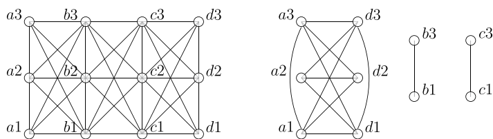
Fig. 11. The graph P_4 \circ P_3 and its strong resolving graph.
