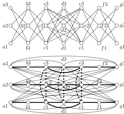
Fig. 8. The direct product H_7 \times K_3 and its strong resolving graph, where H_7 is obtained from a path P_7 = abcdefg by adding the edge ce . According to Theorem 32 , notice that W = \{c, d, e\} . In the strong resolving graph (H_7 \times K_3)_{SR} : the edges in bold correspond to the subgraph H_7 \square N_3 ( N_3 has vertex set \{1, 2, 3\} ); the dashed edges to the subgraph N_3 \square K_3 ( N_3 has vertex set W = \{c, d, e\} ); and the remaining edges to the subgraph ((H_7)_{SR} \circ N_3) \cong (K_3 \circ N_3) ( K_3 has vertex set \{a, d, g\} ).
