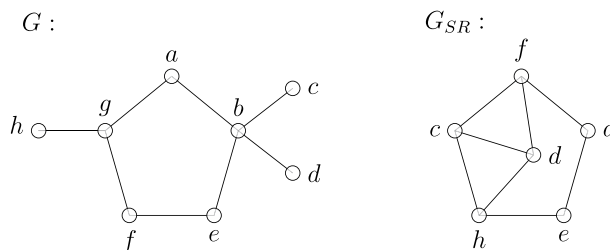
Fig. 4. The set \{a, c, d, h\} \subset V(G) forms a strong metric basis of G . Also, the set \{a, c, d, h\} \subset V(G_{SR}) is a vertex cover of G_{SR} . Thus, \dim_s(G) = \beta(G_{SR}) = 4 .
