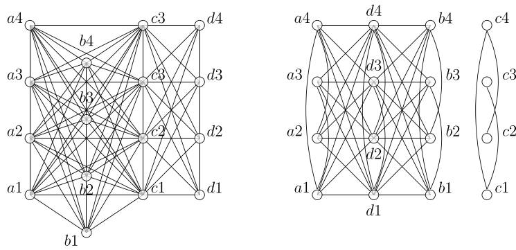
Fig. 12. The graph (K_1 + (K_1 \cup K_2)) \circ P_4 and its strong resolving graph.
