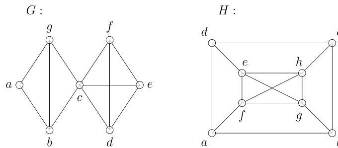
Fig. 1. The set \{d, e, f\} \subset V(G) is composed by true twin vertices in G . Notice that b and g are true twin vertices in G which are not simplicial, while f and d are true twin and simplicial vertices. The set \{e, f, g, h\} \subset V(H) is a twin-free clique in H .
