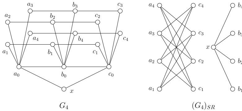
Fig. 5. The graph G_4 \in \mathcal{F} and its strong resolving graph.
