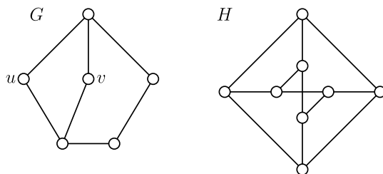
Fig. 9. Two triangle free graphs of diameter two.
