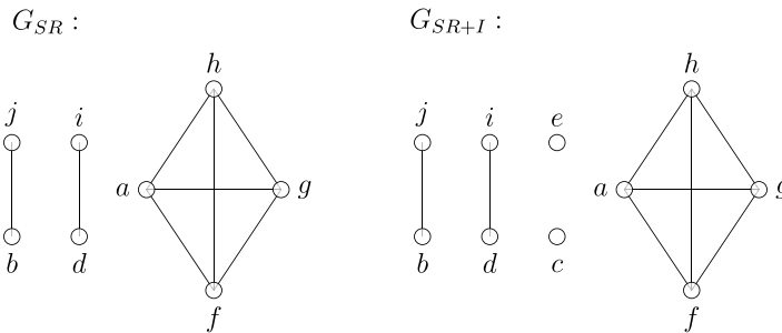
Fig. 3. G_{SR} and G_{SR+I} of the graph G illustrated in Fig. 2.
