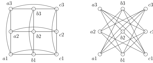
Fig. 7. Cartesian product graph C_3 \square C_3 and its strong resolving graph (C_3 \square C_3)_{SR} .
