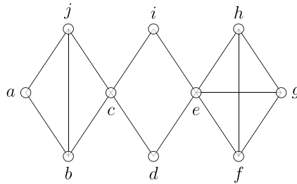
Fig. 2. The set \{a, f, g, h\} is composed by simplicial vertices and its elements are MMD between them. Also, b and j ( d and i ) are MMD. Thus, the boundary of G is \partial(G) = \{a, b, d, f, g, h, i, j\} . Now, M_G(d) = \{a, f, g, h, i\} is the set of vertices which are maximally distant from d . Nevertheless, the vertex d is maximally distant only from the vertex i .
