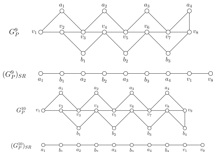
Fig. 6. The graphs G_P^9 and G_P^{10} in \mathcal{F}_P and their strong resolving graphs.
