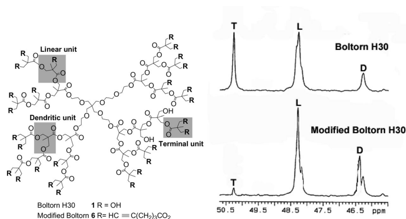
Figure 2. Cq area in the ^{13}\text{C} NMR spectra of dendritic polymers 1 and 6 ; terminal (T), linear (L), and dendritic (D).
