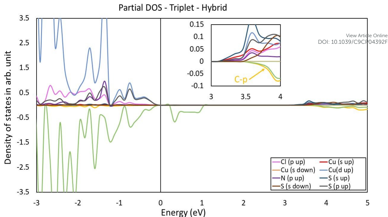
Figure 5: Orbital projected density of states plot (pDOS) for the T_1 Cu-Cy calculated with hybrid (HSE06) density functional theory. The inset shows the amplified view of the conduction band pDOS. The top of the valence band is scaled to 0 eV, also called the Fermi level. The positive and negative density of states here are for spin-up and spin-down channels respectively. The empty band above the valence band is from Cu-3d band, which was not found in S_0 state as presented in Figure 4.
