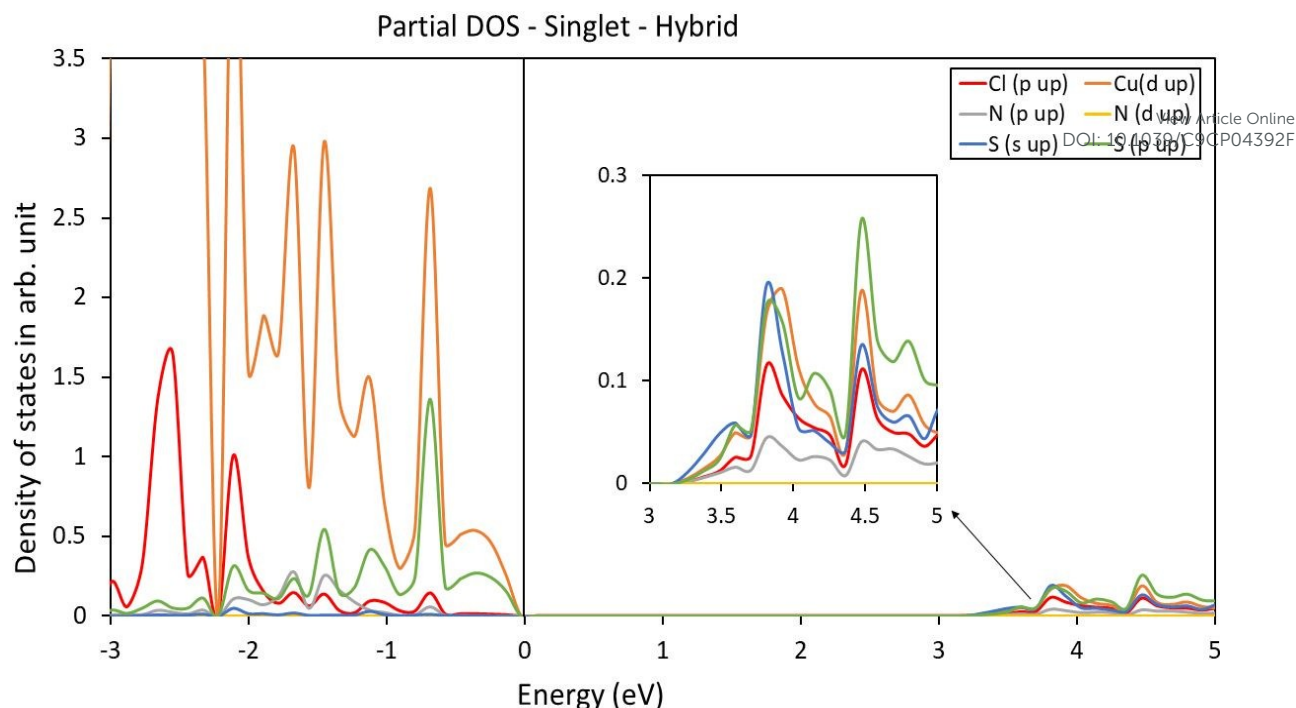
Figure 4: Orbital projected density of states (pDOS) plot for the S_0 Cu-Cy calculated with hybrid density functional theory (HSE06). The inset shows the amplified view of the conduction band pDOS. The top of the valence band is scaled to 0 eV, also called the Fermi level. Even though spin-polarized calculations were performed, as for S_0 states spin-up and spin-down states have exactly the same behavior, so spin-up DOS is plotted here.
