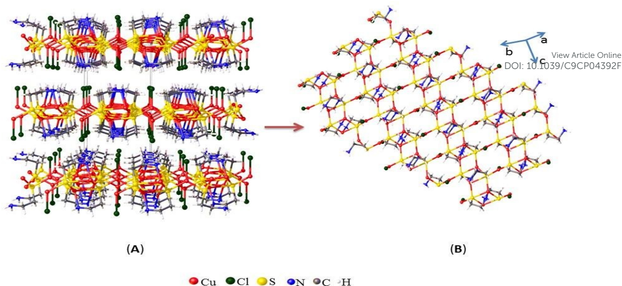
Figure 1. (A) Packing diagram of (1) viewed along (001). (B) Depiction of one strand as part of the unit cell.
