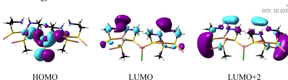
Figure 6. Molecular orbitals involved in the excitation that gives place to the first excited singlet state.
