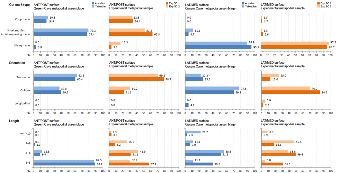
Fig. 2. Bar diagrams showing data on cut mark type, orientation and length in Qesem Cave, and experimental samples. Note that only data from metapodial shafts are shown. Percentages were calculated relative to the total number of cut marks per bone surface [anterior (ANT)/posterior (POST) and lateral (LAT)/medial (MED)].
