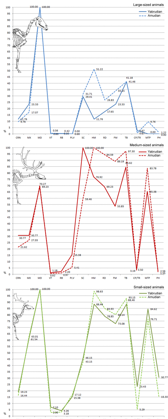
Fig. 1. %MAU distribution by skeletal element and weight size categories split by archaeological contexts (Amudian and Yabrudian). Size classes 5 [very large (<1000 kg)] and 1a [very small (<20 kg)] were excluded, as their low number of elements could lead to distorted outcomes.
