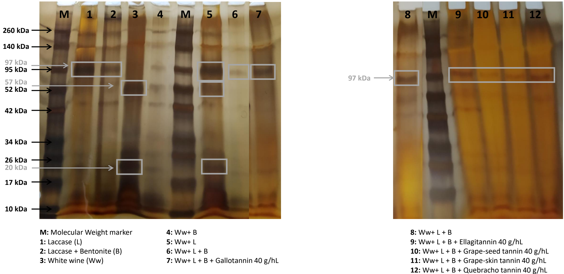
Figure 4. Electrophoresis gels of laccases produced by Botrytis cinerea and supplemented by oenological tannins (40 g/hL) with a bentonite treatment (200 g/hL)
