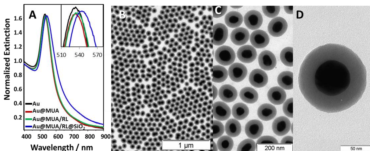
Figure 2. (A) Extinction spectra of Au particles after each step of the presented protocol. (B–D) Representative TEM images at different magnifications of the produced SEPs.
