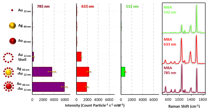
Figure 4. SERS intensity, normalized for a single particle, provided by each material at three laser lines: 785, 633 and 532 nm.
