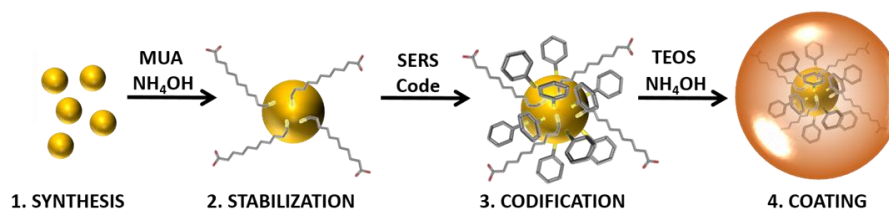
Figure 1. Schematic representation of the MUA assisted encoded process.
