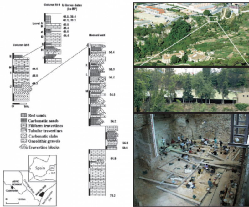
Fig.1: Abric Romaní geographic location and schematic lithostratigraphy of the sequence with the U-Series dates. General view of a part of the “Cinglera de Capello”, front of the site and general view of the excavation in the level M.
