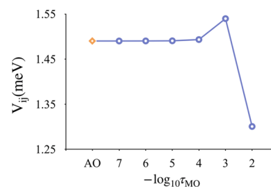
Figure 3. Electronic coupling V_{ij} (in meV) between |S_0S_1\rangle and |T_1T_1\rangle for the pyridine dimer test system as a function of the threshold \tau_{MO} for removing basis functions from the common MO basis. AO refers to the value obtained with the AO basis.
