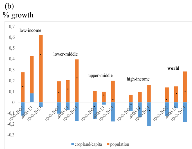
Fig. 1. Changes in cropland demand by income groups, 1990–2013. (a) Changes in total cropland demand, (b) decomposition of changes in cropland demand into population growth and cropland demand per capita according to Eq. (1). The unit in (a) is 1000 km 2 of cropland area harvested and % growth over the entire period 1990–2013, in (b) relative changes in % over each specified period. Note that global cropland is about 15.2 Mkm 2 in 2013, including food and feed provisioning areas reflected here as well as the cropland used for the production of non-food goods and fallowed cropland areas. Note: the dots show the resulting overall change in cropland per capita Source: own elaboration based on FAOSTAT data.
