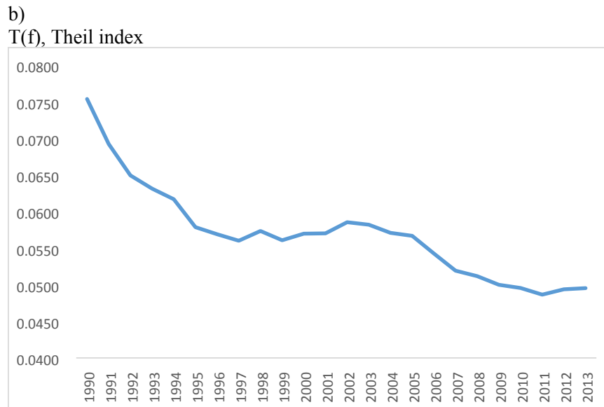
Fig. 3. Food supply per capita. (a) Trajectories of per-capita food supply, as represented by the food index, in the study period 1990–2013 for country groups and the total of all countries, (b) Theil indices of food consumption, given as food index per capita. Units: (a) food index [Mcal/cap/day], (b) dimensionless Theil index of inequality in per-capita food index. Source: own elaboration. Note: in points the estimated trend line (polynomial specification degree 2).
