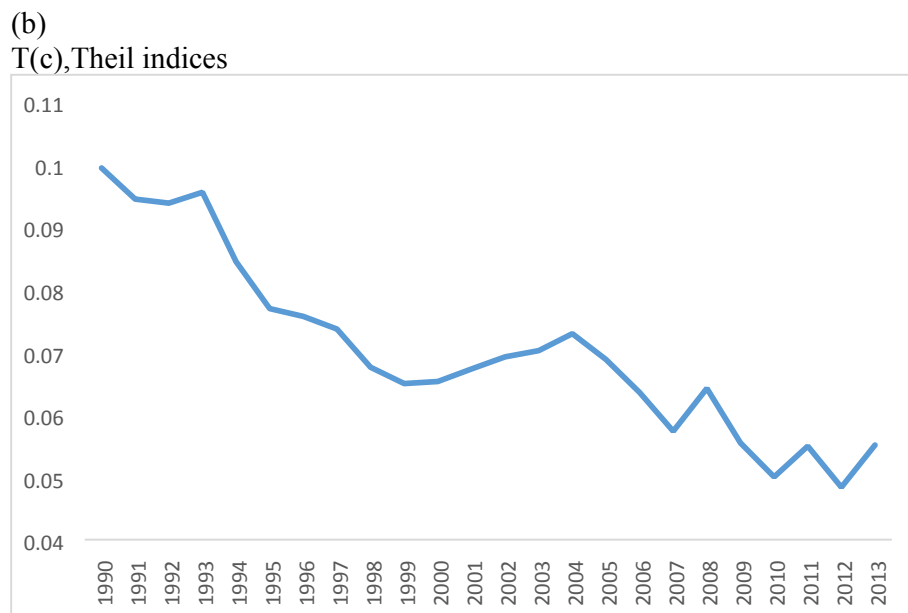
Fig. 2. Trajectories for 1990–2013 of (a) cropland demand per capita and (b) differences of cropland demand per capita between countries in the global average. Units: (a) \text{m}^2/\text{capita} (b) Theil index (dimensionless). Income groups shown in (a) explain 17% of the national-level inequalities analysed in (b). Source: own elaboration based on FAOSTAT data. Source: own elaboration. Note: in points the a trend line (polynomial specification degree 2).
