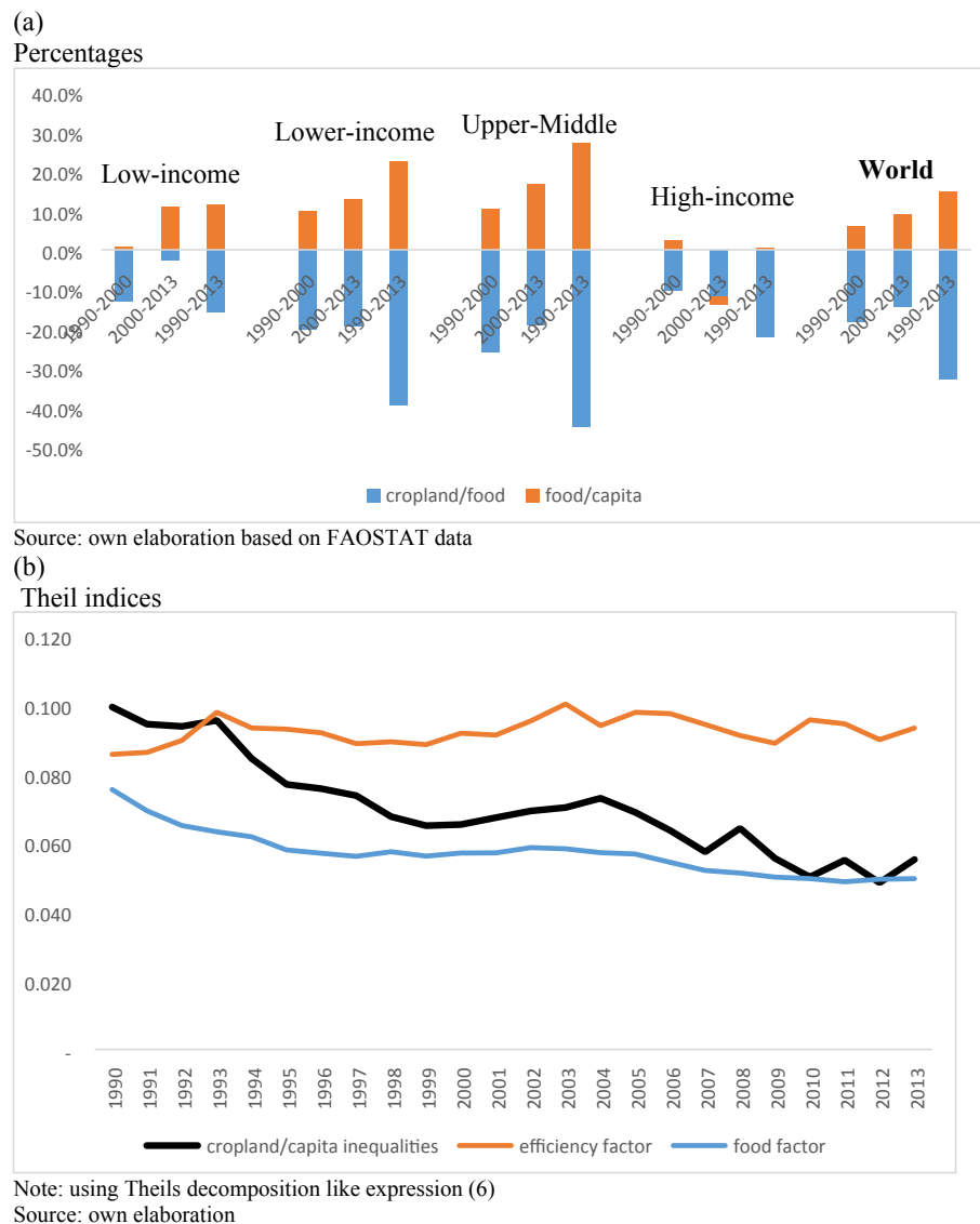
Fig. 5. Decomposition of changes in cropland demand per capita for the period 1990–2013. (a) Decomposition by income groups, (b) trajectory of the cross-country differences as Theil indices of efficiency (cropland demand per food index) and diets (food index per capita). Units are (a) percent changes for each specified period of cropland demand ( \text{m}^2 ) per food index (weighted kcal/cap/day) and food index/capita and (b) inequality in cropland per capita, the efficiency and the food factor, dimensionless Theil indices. Note: using Theils decomposition like expression (6). Source: own elaboration.
