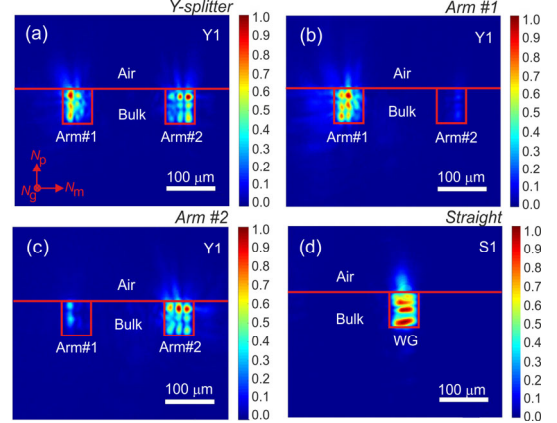
Fig. 13. Near-field laser mode profiles for the Y-branch and straight WGs (Y1 and S1) fs-DLW in Tm:KLuW: (a) Y1, simultaneous operation in both arms (Y-splitter), (b) Y1, operation in arm #1, (c) Y1, operation in arm #2, (d) S1. Red lines – air/crystal interface and WG cladding drawn as a guide for the reader. The laser polarization ( E \parallel N_m ) is horizontal. P_{\text{abs}} = 1.0 \text{ W} , T_{OC} = 50\% .
