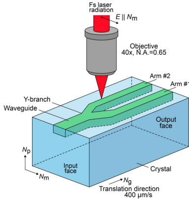
Fig. 1. Scheme of femtosecond direct laser writing of Y-branch waveguides in monoclinic Tm:KLuW crystals: N_p , N_m and N_g – optical indicatrix axes.
