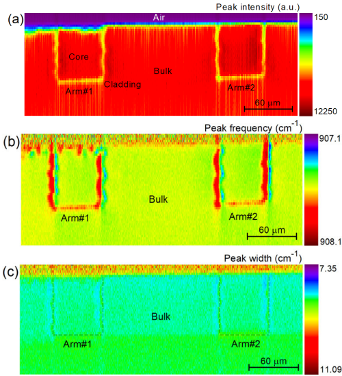
Fig. 7. \mu -Raman mapping of the output facet of the fs-DLW Y-branch WG (Y1) in Tm:KLuW: (a) Raman peak intensity, (b) peak frequency and (c) peak width (FWHM). The mode at \sim 907 \text{cm}^{-1} is monitored. The measurement geometry is g(mm)g (Porto's notations), \lambda_{\text{exc}} = 514 nm.
