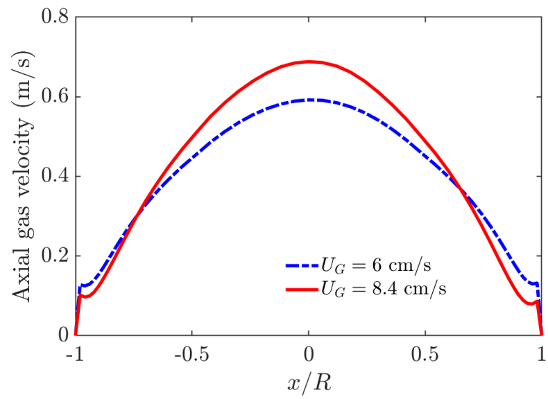
Fig. 4 Time averaged axial gas velocity at superficial gas velocity U_G = 6 cm/s and U_G = 8.4 cm/s.
