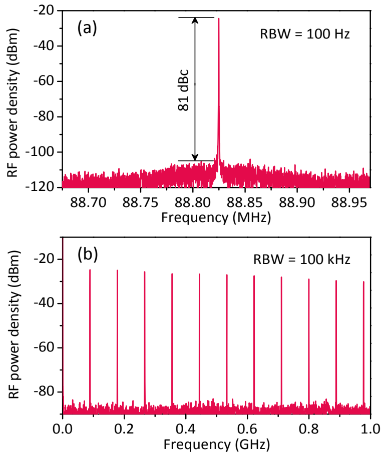
Fig. 5. RF spectra of the GSA mode-locked Tm,Ho:CLNGG laser with external compression: (a) fundamental beat note and (b) 1 GHz span. RBW: resolution bandwidth.
