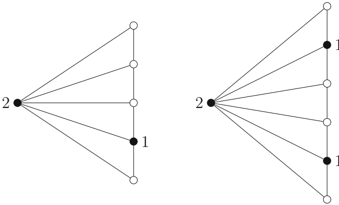
Fig. 3 \gamma_I^s(K_1 + P_5) = 3 and \gamma_I^s(K_1 + P_6) = 4
