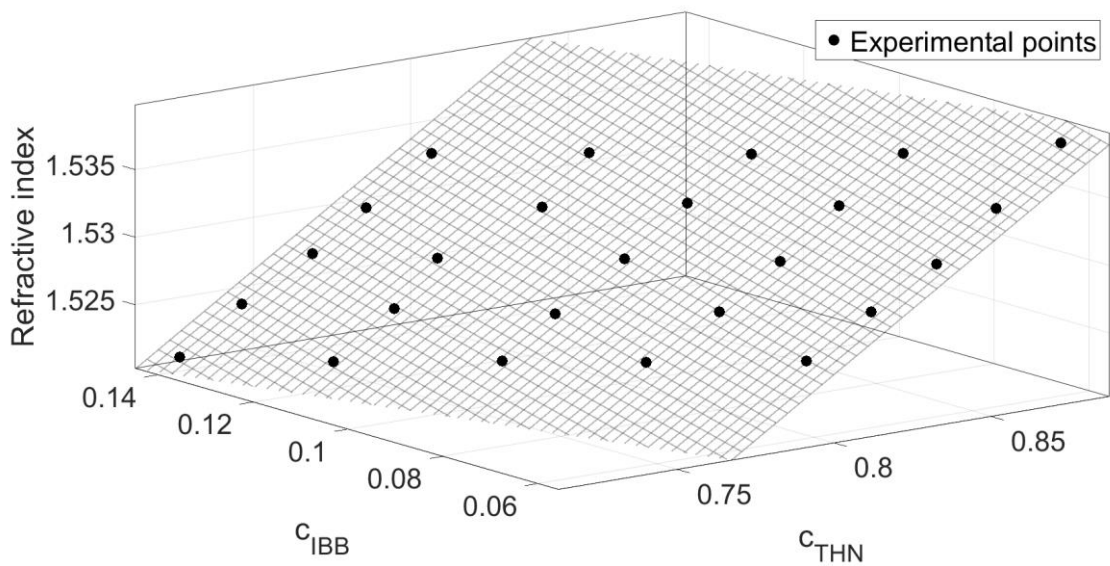
Figure 2: Fitting plane with experimental points from Table 1 at the wavelength of 633nm. C_{IBB} and C_{THN} axes represent mass fraction of isobutylbenzene and tetrahydronaphthalene respectively.
