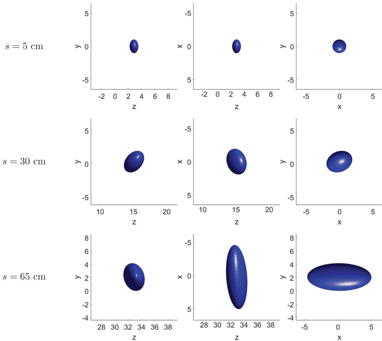
FIG. 6. The three projections on z - y , z - x , and x - y planes of the best-fitting ellipsoid at three different values of traveled distance s = 5, 30, and 65 \text{ cm} corresponding to times t \approx 0.1, 0.24, and 1.0 \text{ s} . All axes in cm.
