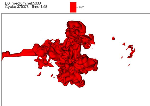
FIG. 9. Video 2: Side x - y view showing the temporal evolution of the \theta = 0.025 isosurface for the DNS of a mild cough. Time is in seconds. Multimedia view: http://dx.doi.org/10.1063/5.0042086.2
