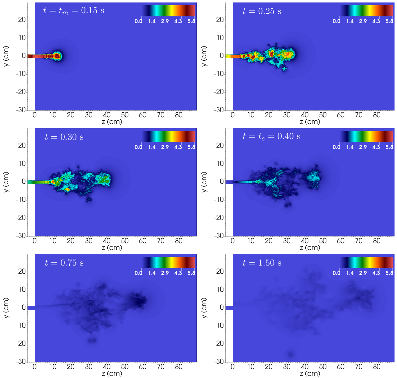
FIG. 2. Detail of the slice at x=0 of the velocity magnitude field (in \text{m s}^{-1} ) at t = 0.15, 0.25, 0.30, 0.40, 0.75, 1.5 s. Note that t = t_m = 0.15 s and t = t_c = 0.40 s correspond to the peak and cough ending times, respectively.
