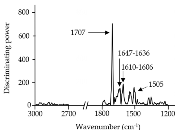
Figure 10. Soft independent modeling of class analogy discriminating power plot of FTIR spectroscopy spectra (3000–2700 \text{cm}^{-1} and 1800–1200 \text{cm}^{-1} ) from a 4-class SIMCA A. diaperinus snack model.
