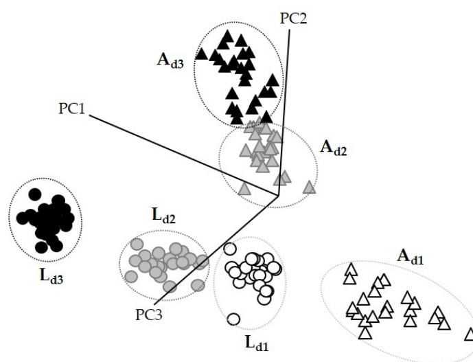
Figure 6. Soft independent modeling of class analogy class projection of FTIR spectroscopy spectra ( 3000\text{--}2700\text{ cm}^{-1} and 1800\text{--}1200\text{ cm}^{-1} ) from a 6-class SIMCA A. diaperinus vs. L. migratoria dough model. Abbreviations used: A d1 , dough with 4.6% of A. diaperinus powder; A d2 , dough with 9.3% of A. diaperinus powder; A d3 , dough with 13.9% of A. diaperinus powder; L d1 , dough with 4.6% of L. migratoria ; L d2 , dough with 9.3% of L. migratoria ; L d3 , dough with 13.9% of L. migratoria .
