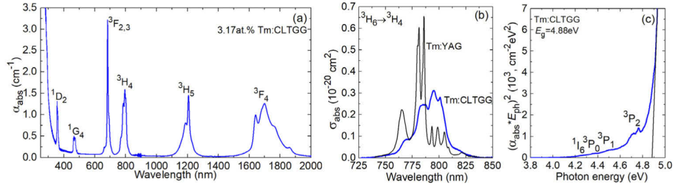
Fig. 6. Absorption of the Tm:CLTGG crystal: (a) RT absorption spectrum; (b) absorption cross-sections, \sigma_{\text{abs}} , for the ^3\text{H}_6 \rightarrow ^3\text{H}_4 \text{Tm}^{3+} transition; (c) Tauc plot for the evaluation of the optical bandgap ( E_g ).
