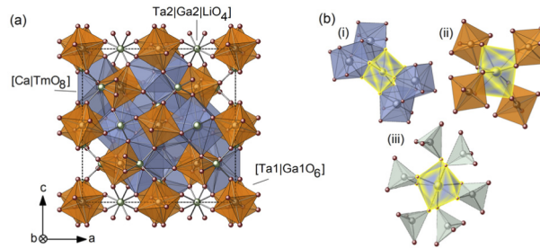
Fig. 3. Crystal structure of Tm:CLTGG: (a) projection of the crystal structure parallel to the a-c plane; (b) the variety of cationic distributions around \text{Ca}^{2+} | \text{Tm}^{3+} ions occupying the dodecahedral 24 c sites: nearest-neighbor cations at: (i) dodecahedral 24 c sites, (ii) octahedral 16 a sites and (iii) tetrahedral 24 d sites.
