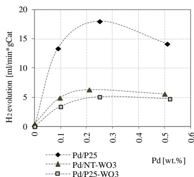
Figure 6. H_2 evolution vs. Pd (wt.%) for Pd/P25, Pd/NT-WO 3 and Pd/P25-WO 3 catalysts, varying the amount of Pd deposited. Experimental conditions: catalysts 166.67 ppm, 600 ml of a water-methanol (50 vol.%) solution under simulated solar light (Xe Lamp, 300-800 nm, 250 W/m 2 , I_{250-450nm} : 6.5 \times 10^{-4} Einstein/min). Pd incorporation by PD-2m10.
