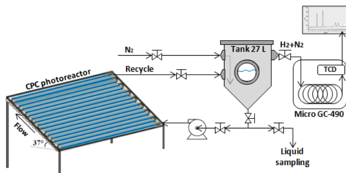
Figure 1. Experimental set up of photocatalytic H 2 generation in the pilot-scale solar reactor.
