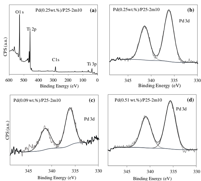
Figure 4. XPS full spectra of the catalysts (a). High-resolution XPS spectra of Pd 3d (b,c, d) spectral region of Pd/P25 catalysts.
