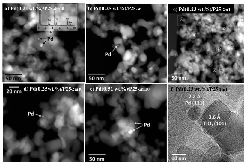
Figure 3. STEM-HAADF images for Pd/P25 catalysts, where Pd was deposited by a) PD 4m10; b) wetness impregnation; c) PD 2m1; d) 2m10, e) PD 2m10, and f) 2m1
