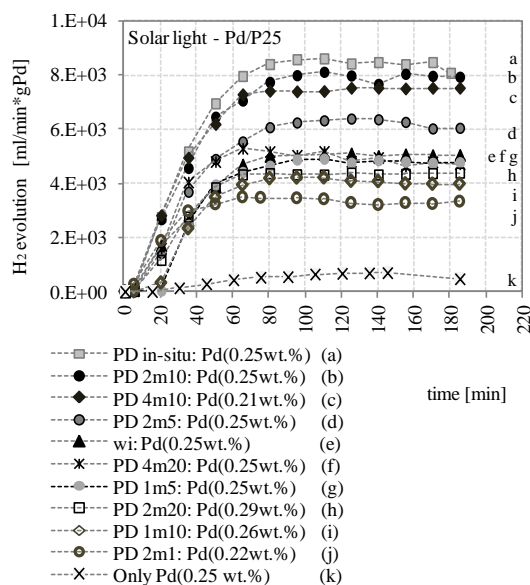
Figure 5. H 2 generation for Pd/P25 varying the Pd deposition method. Experimental conditions: catalysts 167 ppm, 600 ml of a water-methanol (50 vol.%) solution under simulated solar light (Xe Lamp, 300-800 nm, 250 W/m 2 , I 250-450nm : 6.5x10 -4 Einstein/min).
