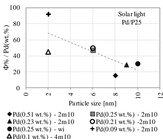
Figure 8. Effect of Pd particle size on quantum yield ( \Phi\% / \text{Pd}(\text{wt.}\%) ) for different Pd/P25 catalysts. Experimental conditions: catalysts 166.67 ppm, 600 ml of a water-methanol (50 vol.%) solution under simulated solar light (Xe Lamp, 300-800 nm, 250 W/m 2 , I 250-450nm : 6.5x10 -4 Einstein/min).
