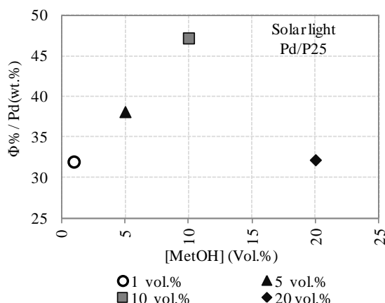
Figure 9. Effect of methanol concentration -in the Pd photodeposition- on quantum yield ( \Phi % / Pd(wt.%)) for different Pd(0.25 wt.%) / P25 catalysts. Experimental conditions: catalysts 166.67 ppm, 600 ml of a water-methanol (50 vol.%) solution under simulated solar light (Xe Lamp, 300-800 nm, 250 W/m 2 , I 250-450nm : 6.5x10 -4 Einstein/min). Pd incorporation by PD-2mX.
