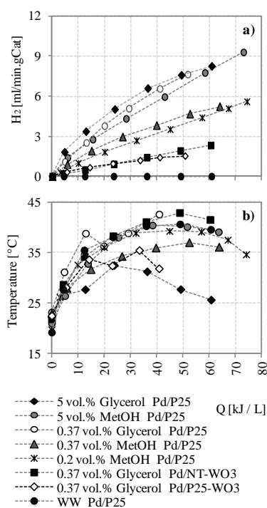
Figure 7. H 2 evolution vs. accumulated solar UV energy for Pd (0.25 wt.)/P25 in water- methanol and -glycerol mixtures. Experimental conditions: catalysts 200 ppm in 25 L under solar light. WW: municipal wastewater from Almería, Spain.
