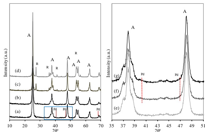
Figure 2. XRD patterns. a) Pd(0.5 wt.%)/NT-WO 3 -2m10; b) Pd(0.21 wt.%)/NT-WO 3 -2m10; c) Pd(0.52 wt.%)/P25-WO 3 -2m10; d) Pd(0.51 wt.%)/P25-2m10; e) NT-WO 3 ; f) Pd(0.21 wt.%)/NT-WO 3 -2m10; g) Pd(0.35 wt.%)/NT-WO 3 -2m10
