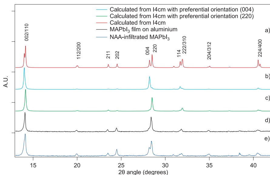
FIGURE 4 Calculated diffractograms of \text{MAPbI}_3 from the tetragonal structure ( I4cm , a 8.849; b 8.849, c 12.642; at 293K) with no preferential orientation (red line), preferential orientation toward the (004) plane (blue line), preferential orientation toward the (220) plane (green line), and experimental diffractogram of the \text{MAPbI}_3 layer deposited on bare aluminum substrates (black line)
