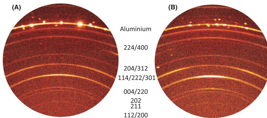
FIGURE 5 2D area images of grazing incidence XRD of the MAPbI 3 layer deposited on bare aluminum substrates (A) and infiltrated in NAA layers (B). The Debye rings are indexed with the diffraction planes
