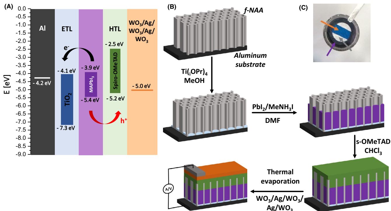
FIGURE 1 A, Band diagram of the NAA-PSC device fabricated in this study; (B) schematic depiction of the solar cell device fabrication; (C) picture of an actual device, the purple arrow points to the MAPbI 3 layer, the orange arrow points to the semitransparent anode, while the gray arrow points to the silver upper contact
