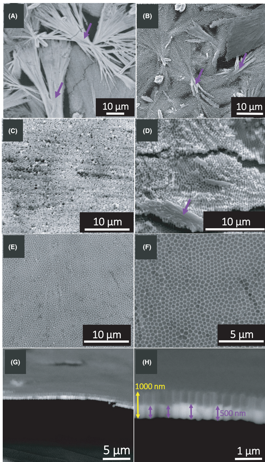
FIGURE 3 SEM images of NAA substrate filled with MAPbI 3 via spin-coating using a precursors concentration of 2.5 mol L -1 (A, B), 1.5 mol L -1 (C, D), and 2.0 mol L -1 (E, F). The MAPbI 3 layer is shown by the purple arrows. Pictures (G, H) are cross-section SEM images of the layers depicted in pictures (E, F) recorded with a backscattered electrons detector, where the brightness is proportional to the presence of higher atomic number elements. The MAPbI 3 layer is shown by the purple arrows while the yellow arrows show the pores' height. The scales are indicated in each picture
