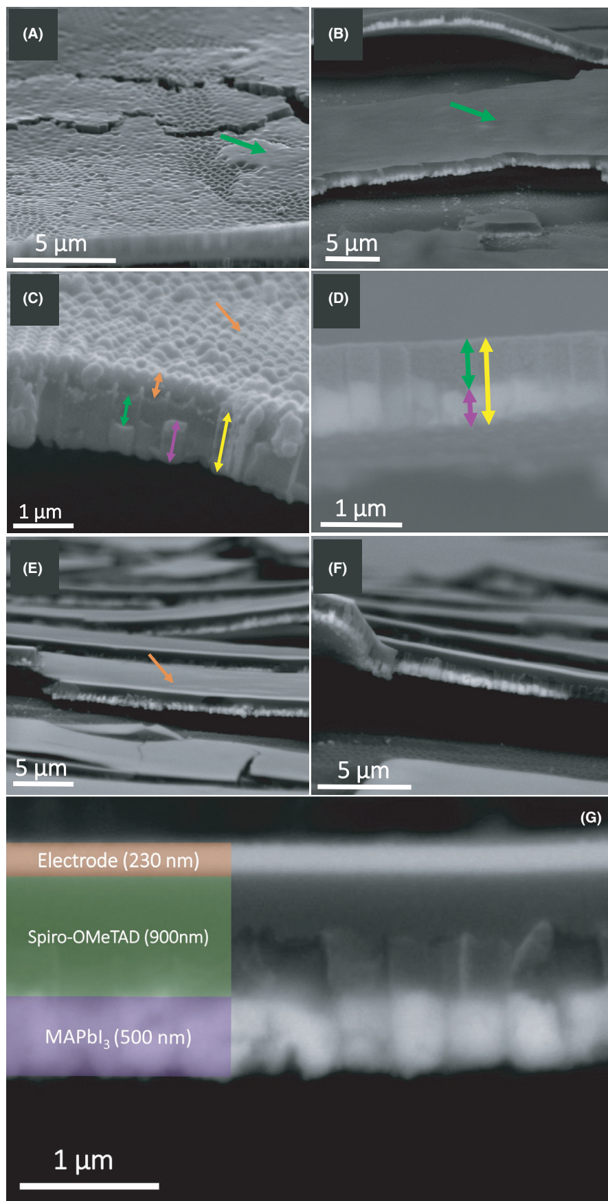
FIGURE 7 A, SEM image of NAA substrate filled with MAPbI 3 (via spin-coating using a precursors concentration of 2.0 mol L -1 ) with inhomogeneous coverage with a spiro-OMeTAD layer. B, SEM image of NAA substrate filled with MAPbI 3 with homogeneous coverage with a spiro-OMeTAD layer (backscattered electrons detector). C, Cross-section SEM image of the afore-mentioned sample. D, SEM image of NAA substrate filled with MAPbI 3 with inhomogeneous coverage of spiro-OMeTAD and upper WO 3 /Ag anode. E-G, SEM images of a complete NAA-PSC device. The MAPbI 3 , spiro-OMeTAD and the semi-transparent electrode layers are marked by purple, green and orange arrows, respectively. The yellow double arrow denotes the pores thickness. The scales are indicated in each picture
