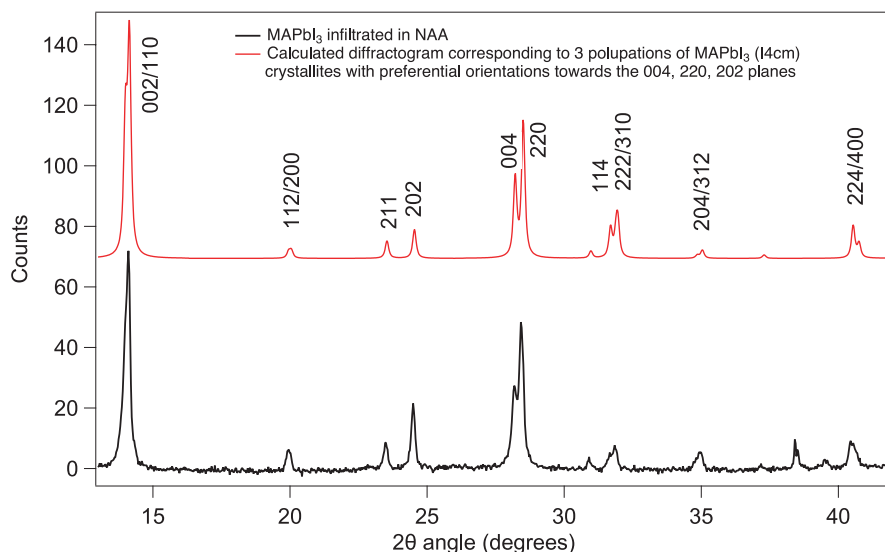
FIGURE 6 Sum of calculated diffractogram of MAPbI 3 from the tetragonal structure (I4cm, a 8.849; b 8.849, c 12.642; at 293K) with preferential orientation (preferential orientation toward the (004), (220), and (202) planes with 34%, 55%, and 11% respective contributions (red line), and experimental diffractogram of the MAPbI 3 layer deposited on NAA substrates (black line)
