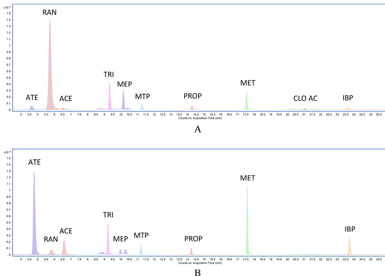
Fig. 3. Chromatograms obtained when a non-spiked sample of river water (A) and effluent wastewater (B) was analysed by SPE/LC-MS/MS.
