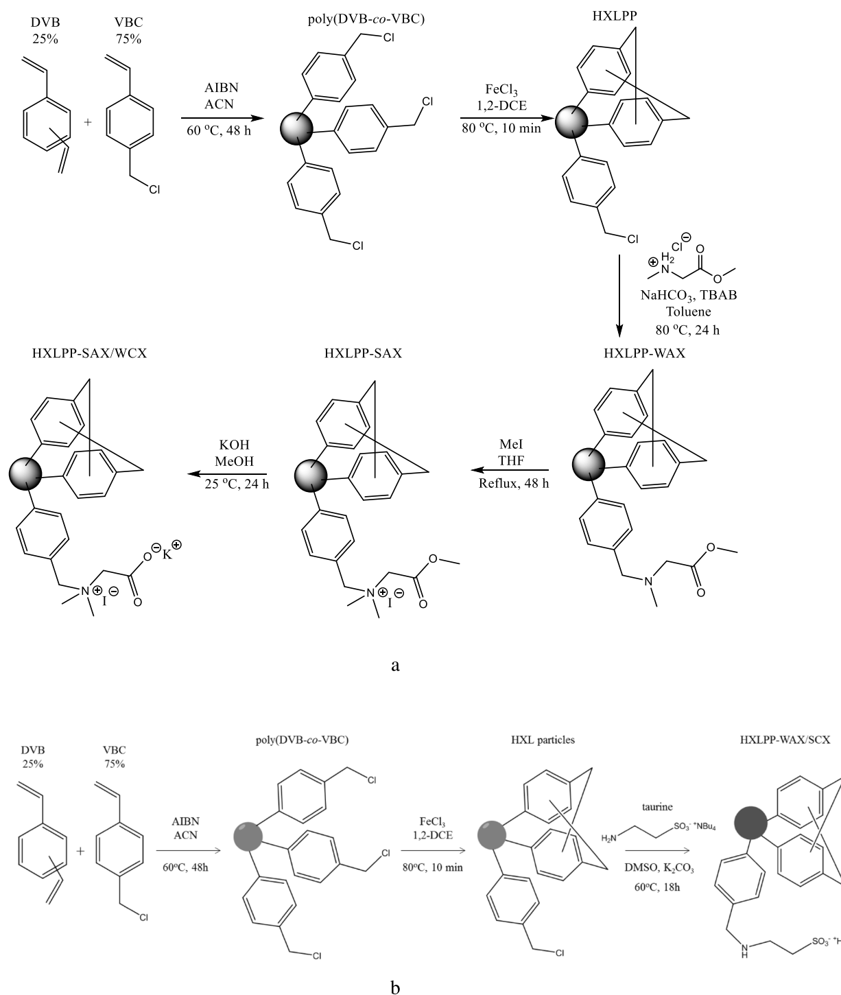
Fig. 1. Reaction schemes showing the synthetic methods used to prepare the HXLPP-SAX/WCX sorbent (a) and the HXLPP-WAX/SCX sorbent (b).
