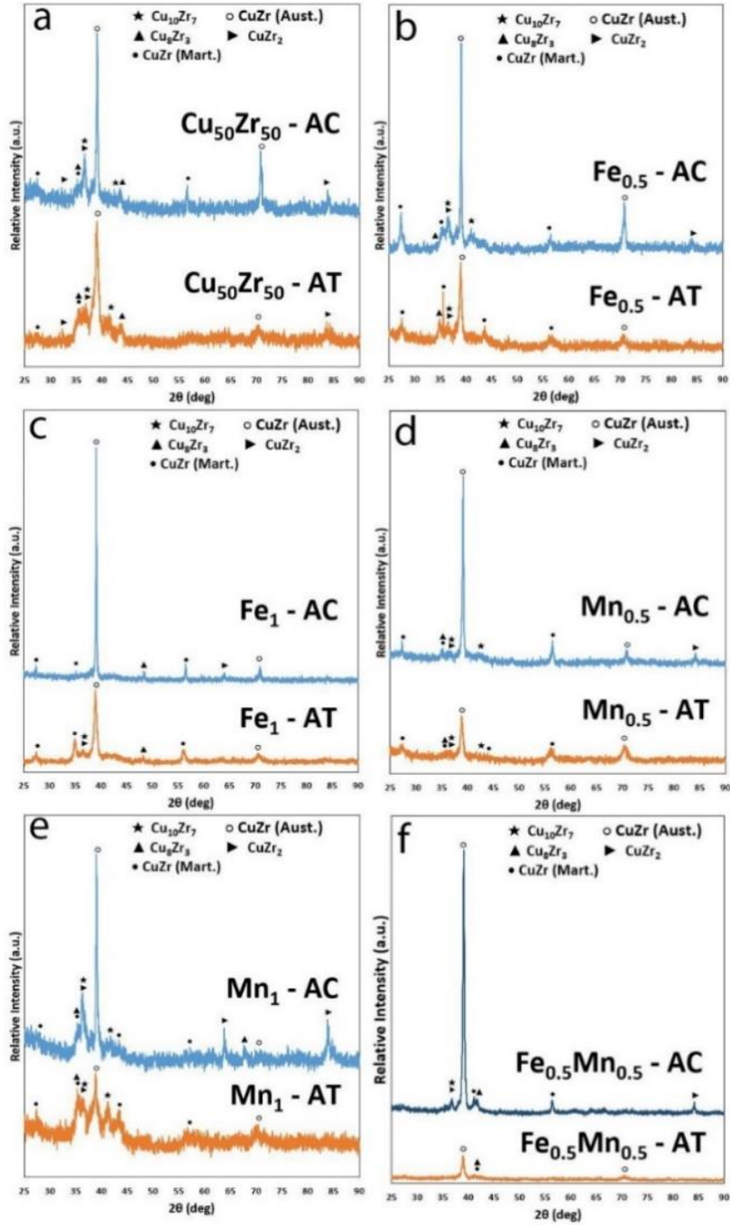
Fig. 10. XRD scan of 2 mm diameter as-cast (AC) and after wear tested (AT) alloys with 15 N load for (a) \text{Cu}_{50}\text{Zr}_{50} , (b) \text{Cu}_{49.5}\text{Zr}_{50}\text{Fe}_{0.5} , (c) \text{Cu}_{49}\text{Zr}_{50}\text{Fe}_1 , (d) \text{Cu}_{49.5}\text{Zr}_{50}\text{Mn}_{0.5} and (e) \text{Cu}_{49}\text{Zr}_{50}\text{Mn}_1 and (f) \text{Cu}_{49}\text{Zr}_{50}\text{Fe}_{0.5}\text{Mn}_{0.5} .
