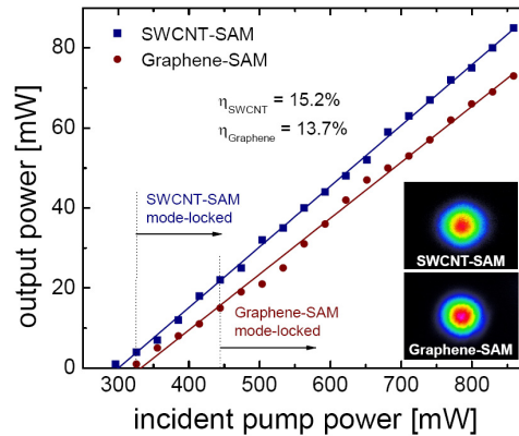
Fig. 3. Average output power of the Yb:KLuW laser mode-locked by SWCNT-SAM (squares) and graphene-SAM (circles) with 1% output coupling and the beam profiles recorded for both SAMs in mode-locked operation (inset). \eta denotes slope efficiency.
